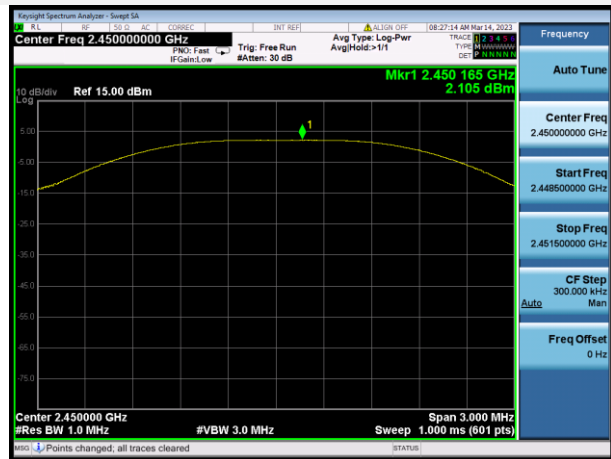
FSK MIDDLE CHANNEL
