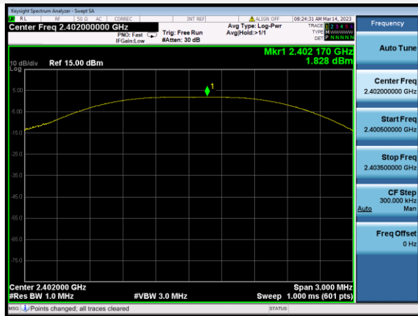
FSK LOW CHANNEL
