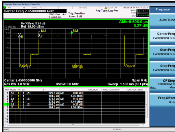
FSK(1Mbps)
