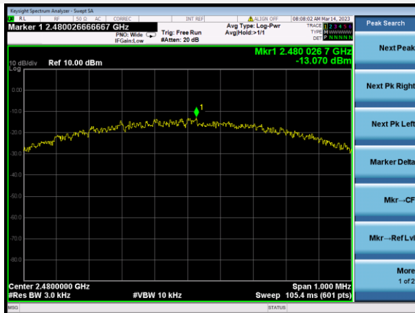
FSK HIGH CHANNEL
