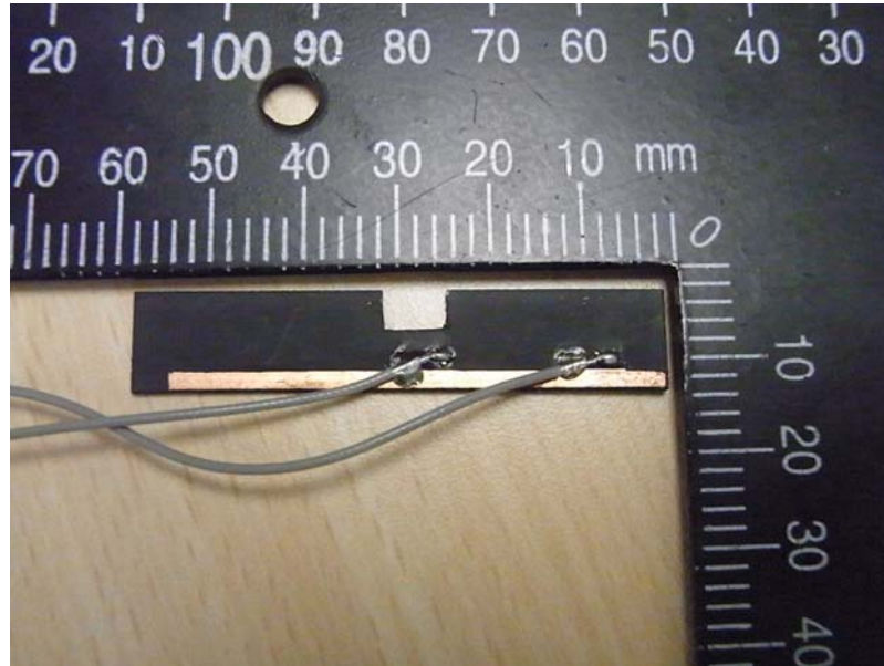
Front View of WLAN/Bluetooth Antenna(Aux.)
