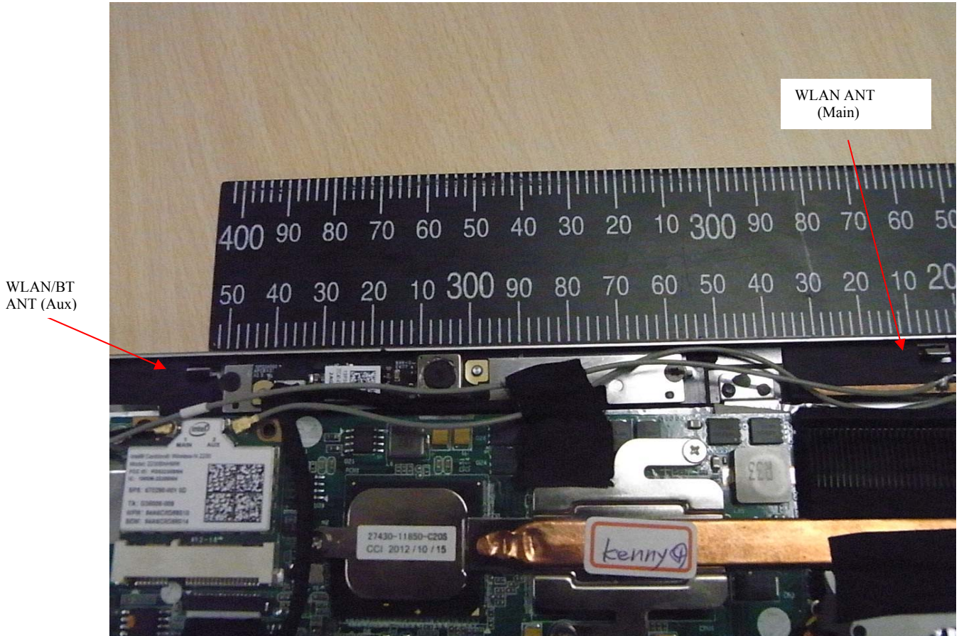
EUT (Main and Aux) Transmit Antenna Location
