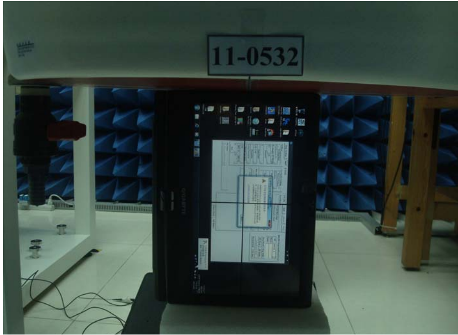
Figure 2. Body SAR Test Setup (Edge Left to phantom)
