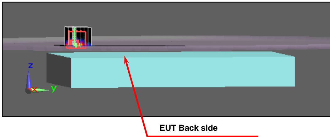
Figure 1. Body SAR Test Setup (Back Surface to phantom)
