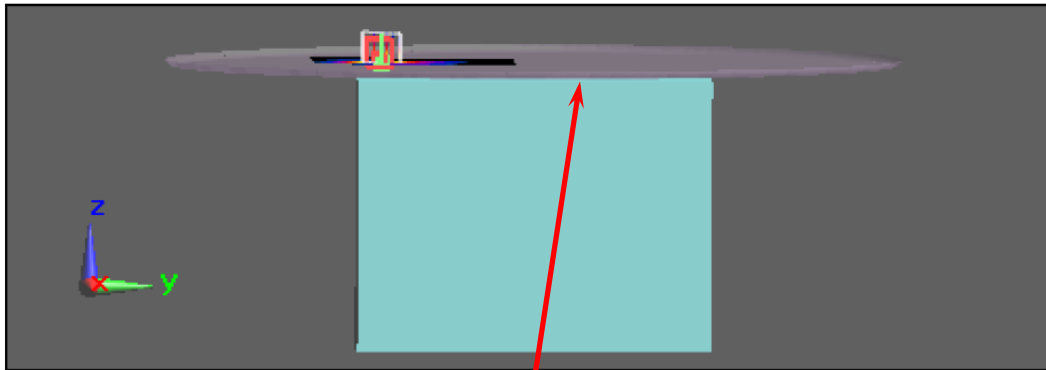
Figure 3. Body SAR Test Setup (Edge Top to phantom)
