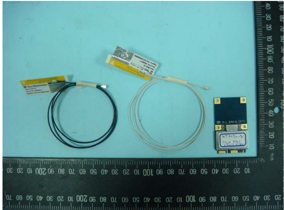
EUT 1: Full Size Module with two Antenna Connectors
