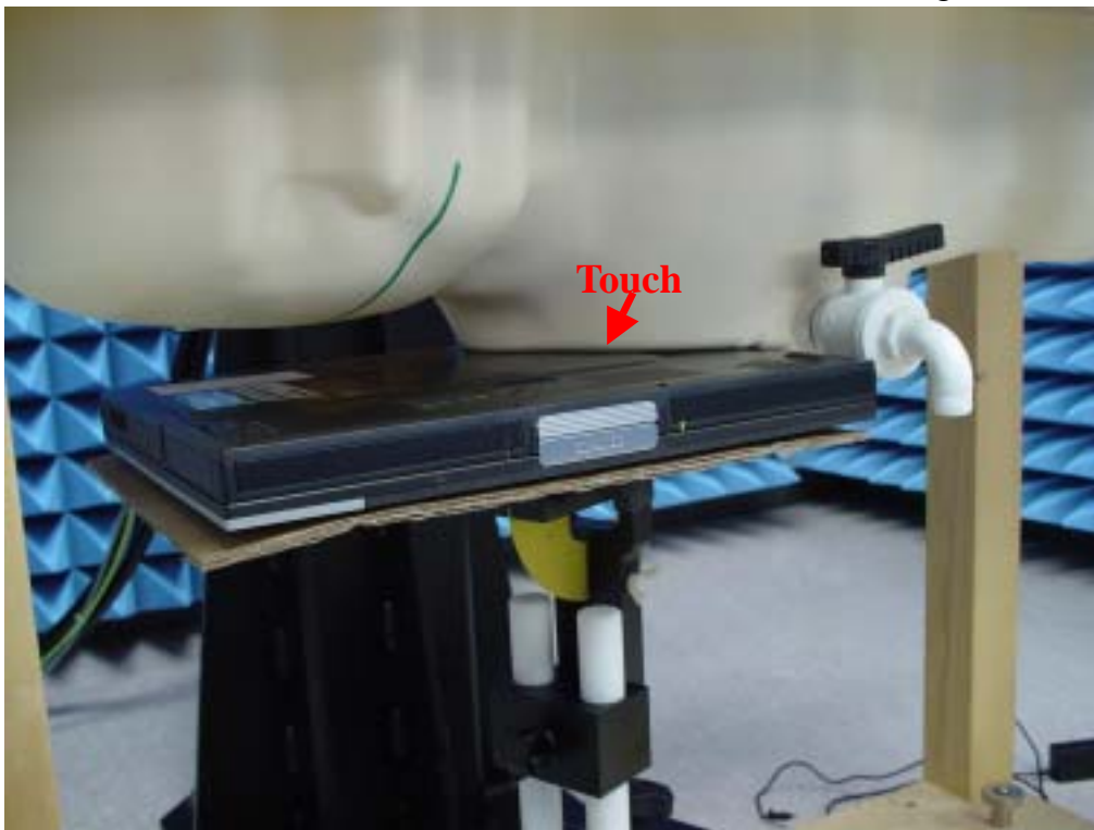
Fig.6 Photograph of the top cover parallel and at a distance of 0.0 cm from the base of the phantom.
