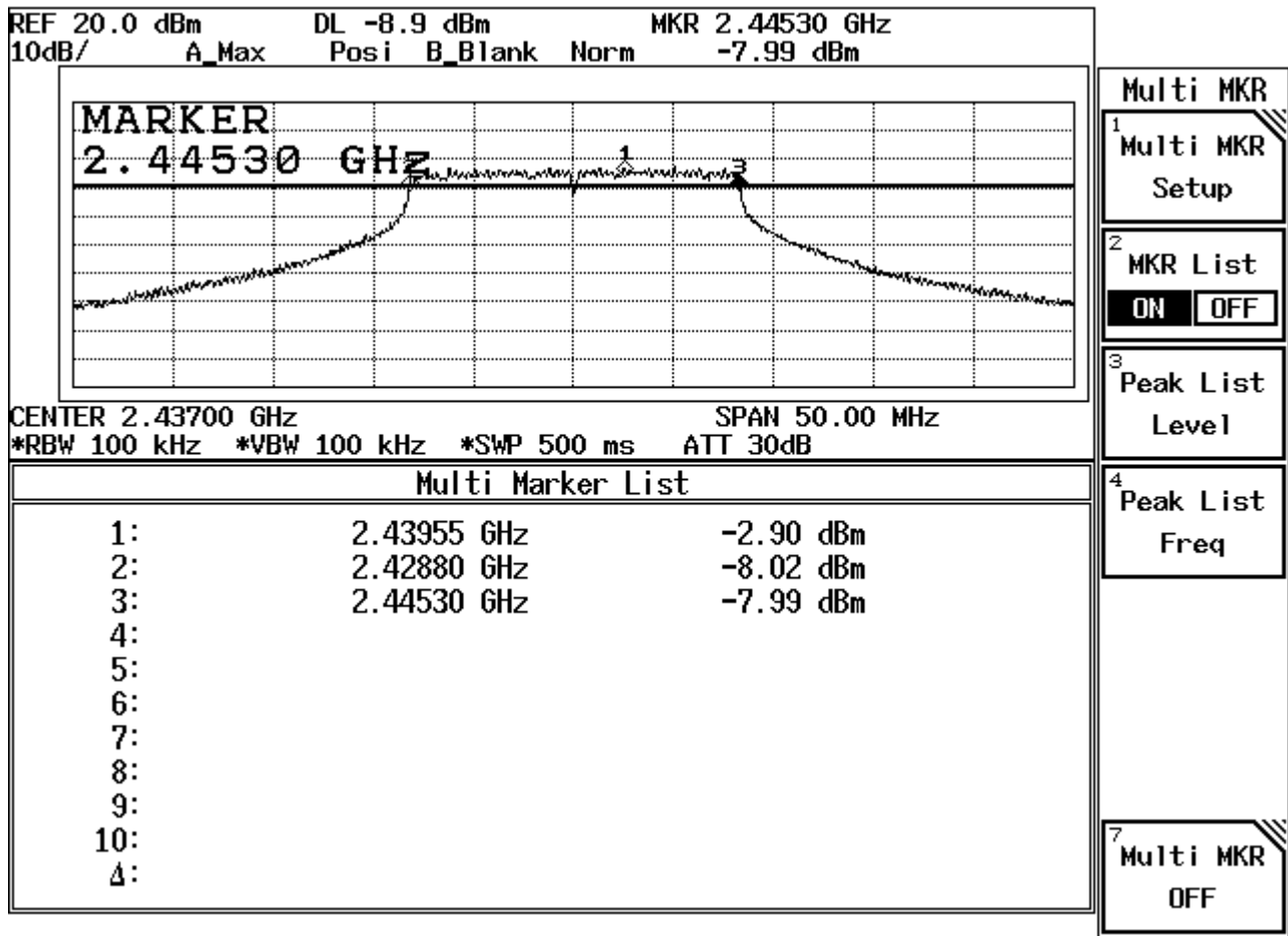
Figure Channel 6: 54Mbps
