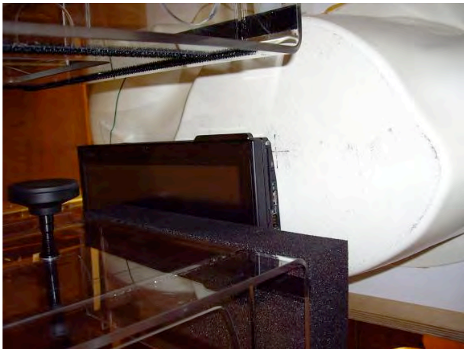
Figure 12-4 Notebook positioned under flat section of phantom
