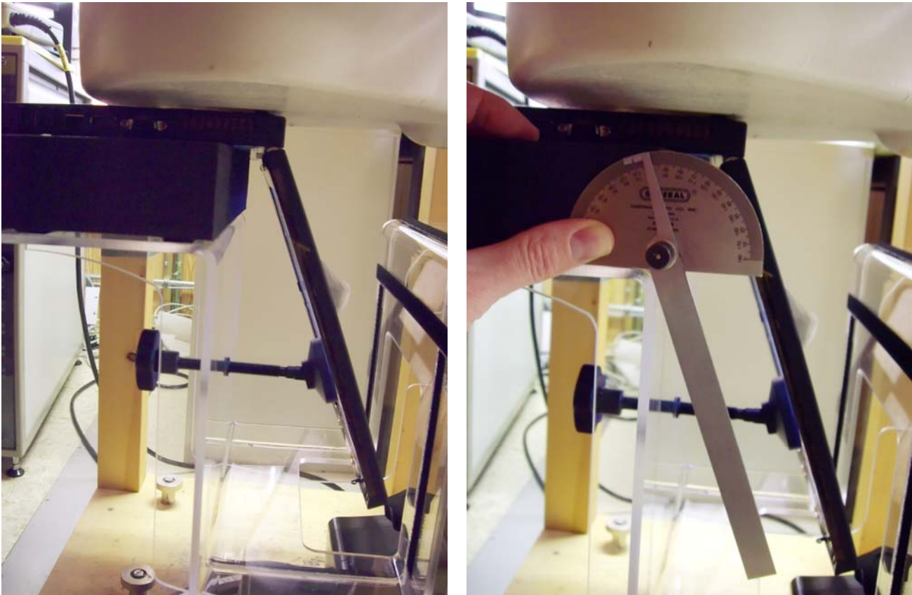
Figure 12-4 Notebook positioned under flat section of phantom
