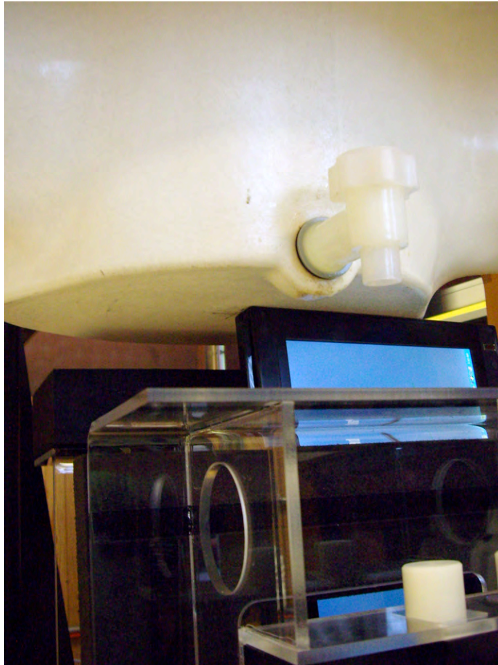
Figure 11-6 Notebook positioned under flat section of phantom, Secondary Portrait position (view 1)
