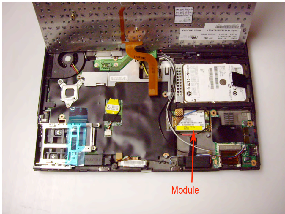
Figure 11-4 Internal View of Notebook Showing Module Location
