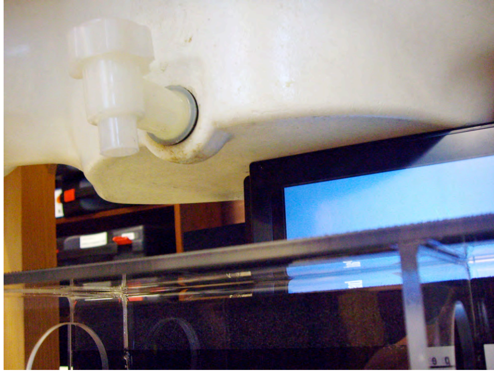
Figure 11-7 Notebook positioned under flat section of phantom, Secondary Portrait position (view 2)
