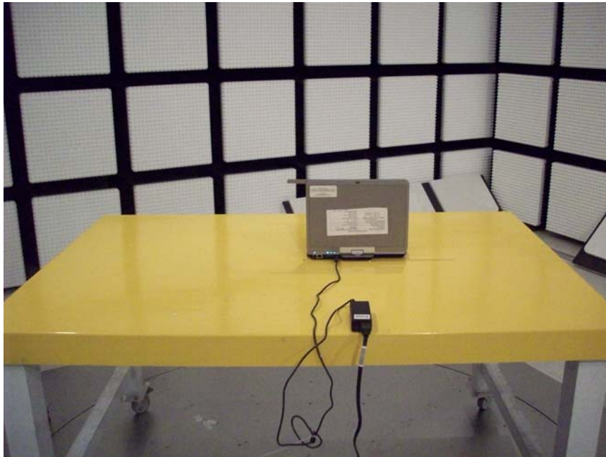
MOBILE ANTENNA AT 180 DEGREES BACK
