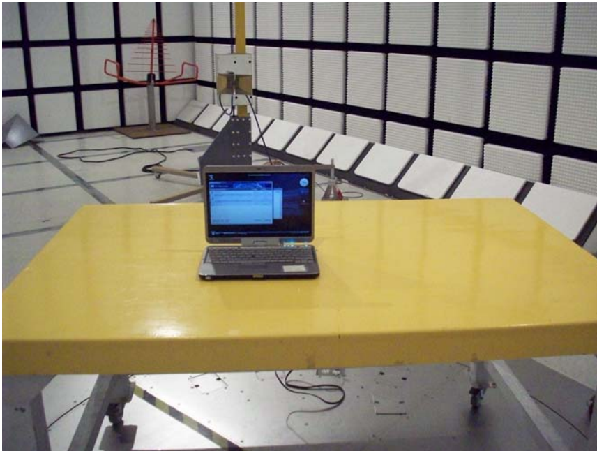
MOBILE ANTENNA AT 180 DEGREES FRONT
