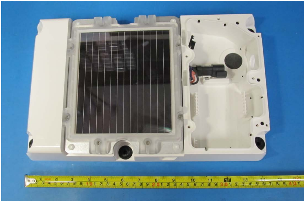
Figure 1 TT210 Top View
