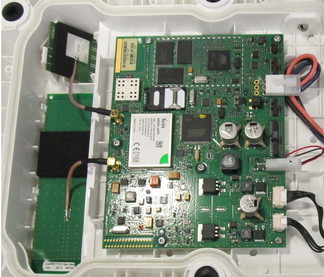
Figure 3 PCB Detail
