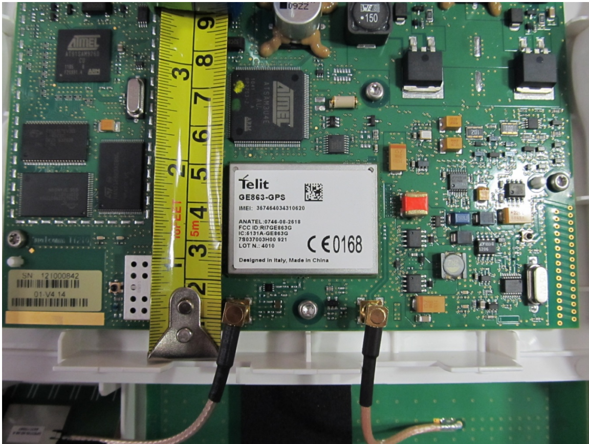
Figure 4 GSM Module Detail (shield on)
