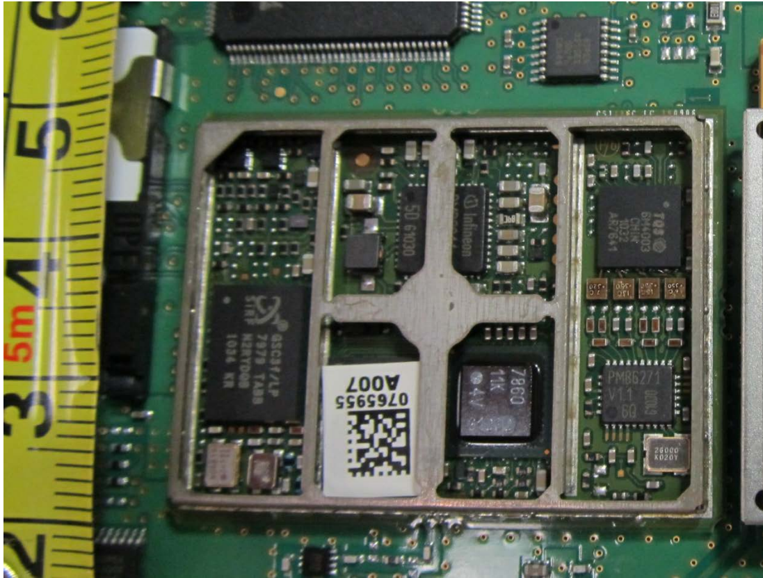
Figure 6 GSM Module Detail (Shield Off)
