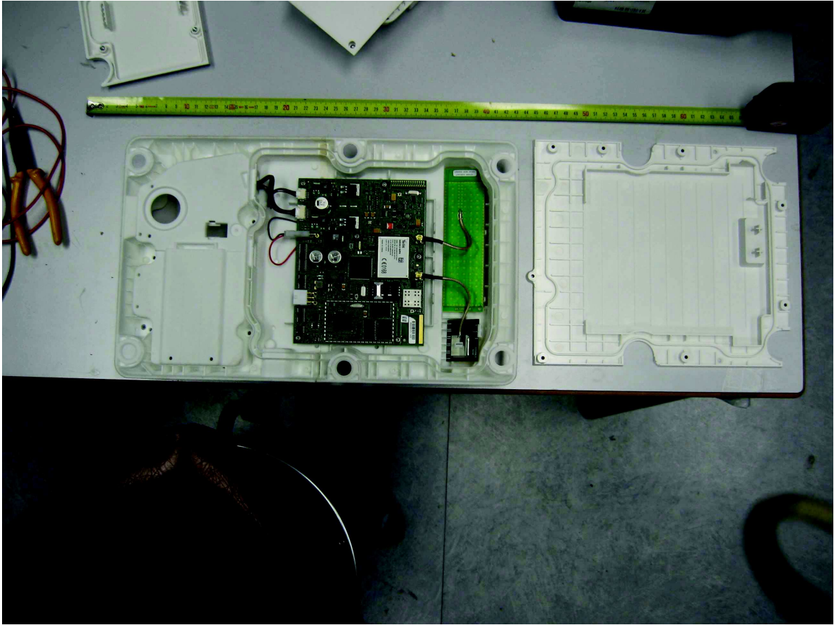
Bottom view without plastic cover
