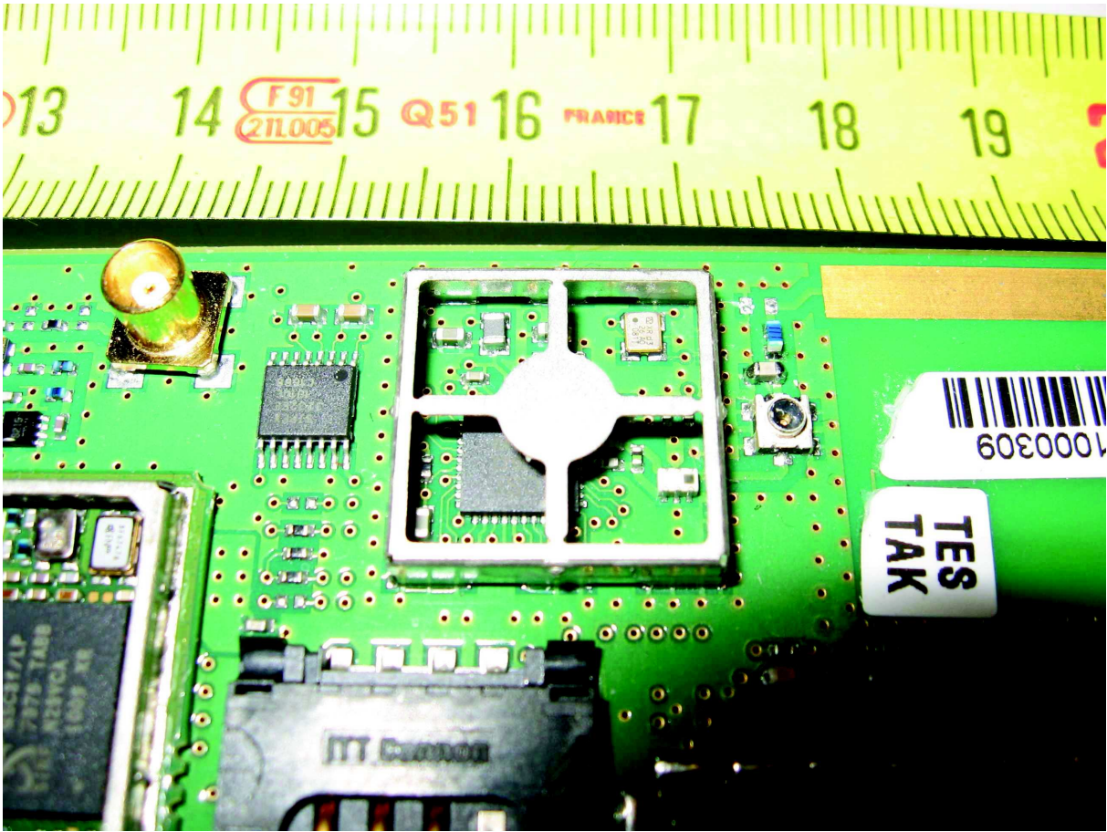
BT radio
