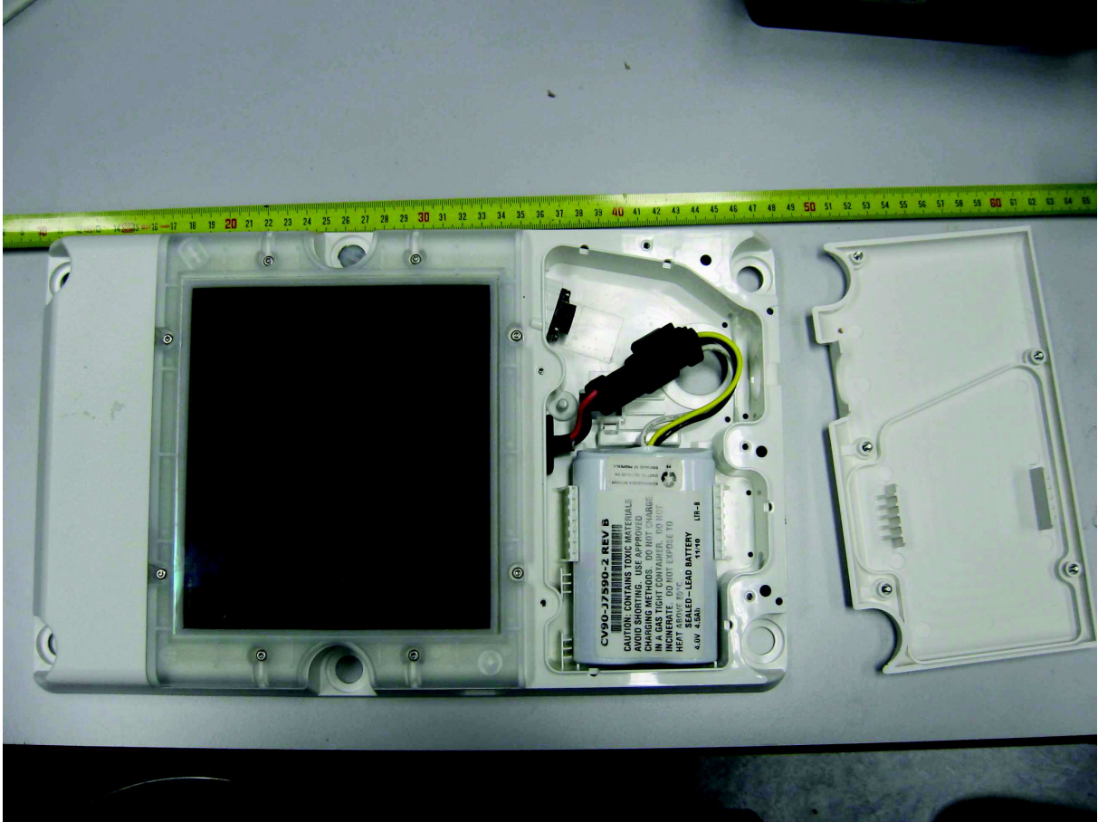
Battery location and connectors for I/O
