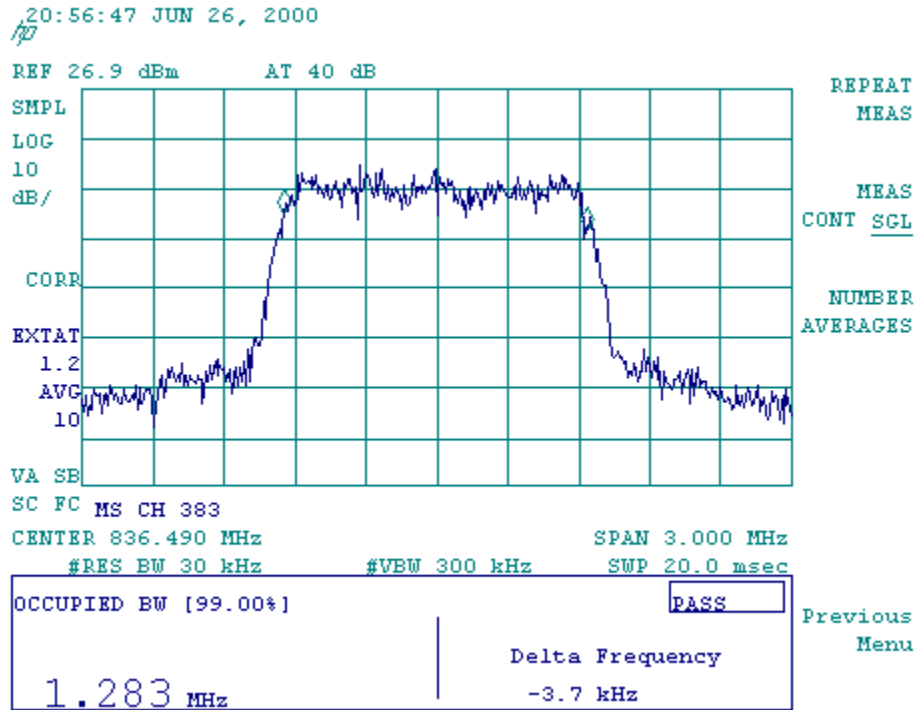
99% Occupied Bandwidth
