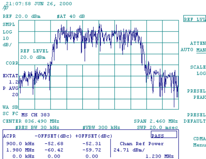
ACPR (Adjacent Channel Power Ratio)
