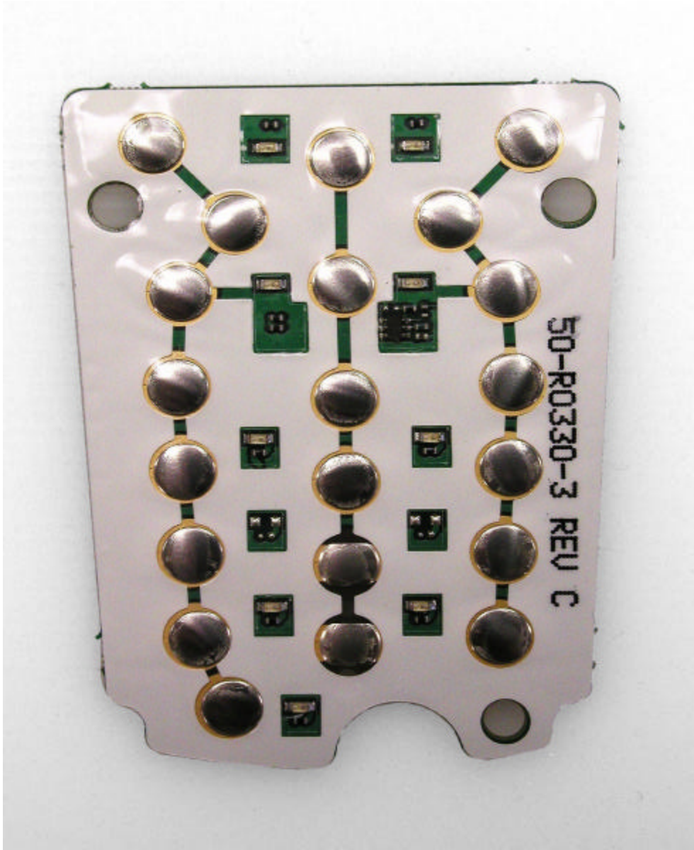
Keyboard with dome layer
