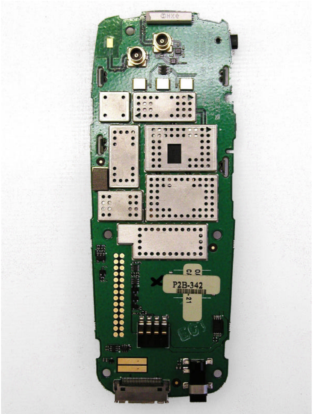
Main board rear view
