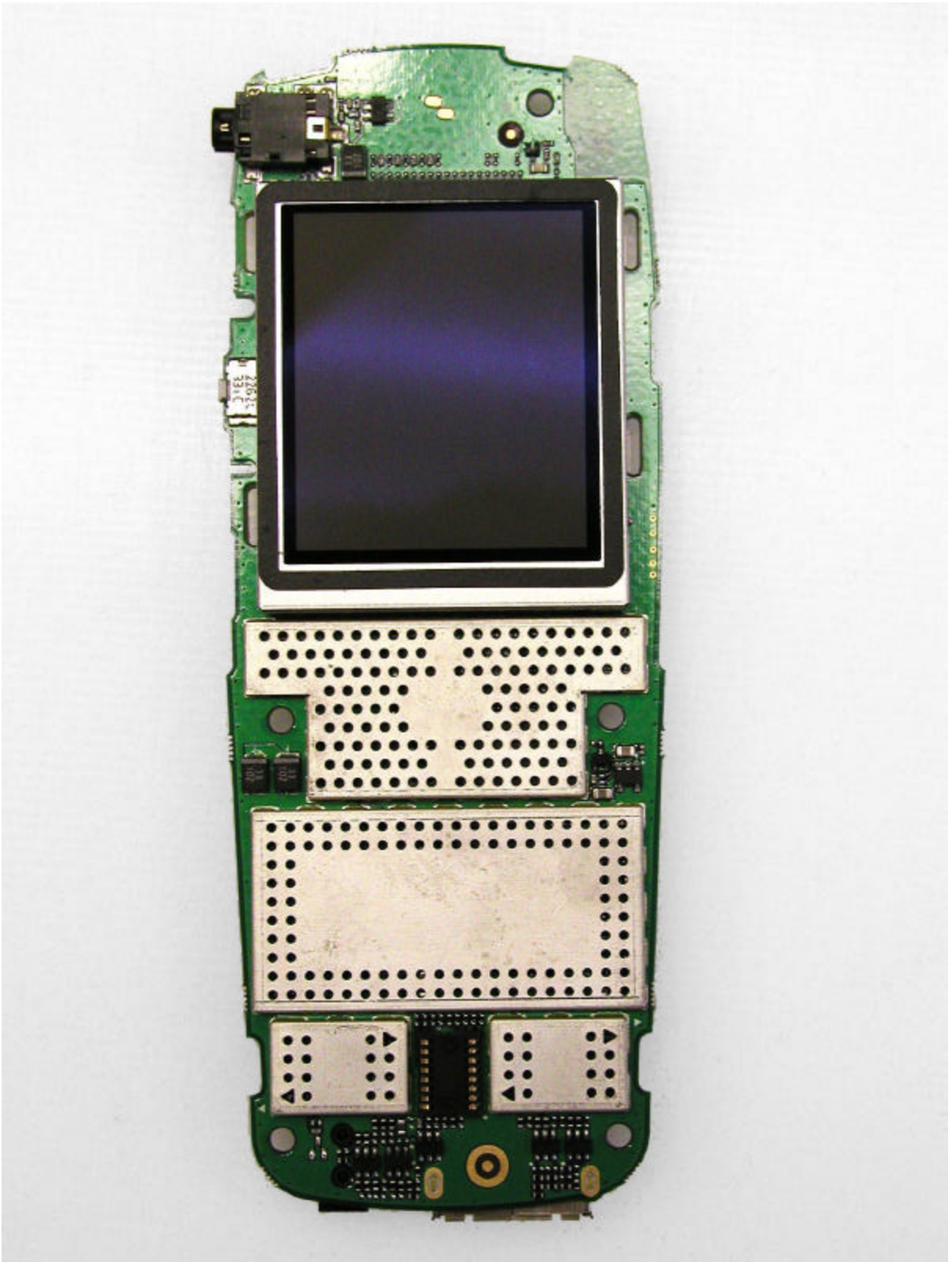
Main board front view
