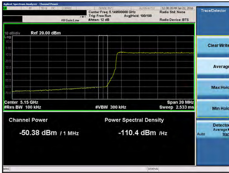
Plot 7-29. Conducted Average Band Edge Plot (LAA (UNII Band 1, 20MHz BW) – Ch. 46890)
