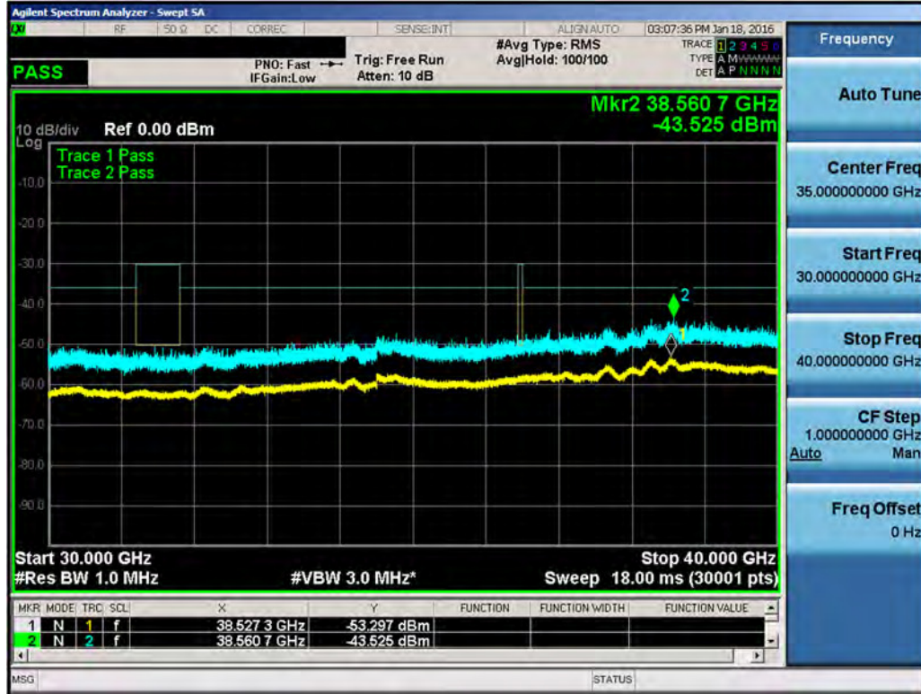
Plot 7-97. Conducted Spurious Plot (LAA (UNII Band 3, 20MHz BW) – Ch. 53540)
