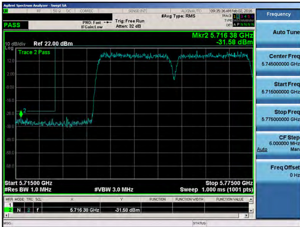
Plot 7-38. Conducted Peak Band Edge Plot #1 (LAA (UNII Band 3, 40MHz BW) – Ch. 52740, 52940)
