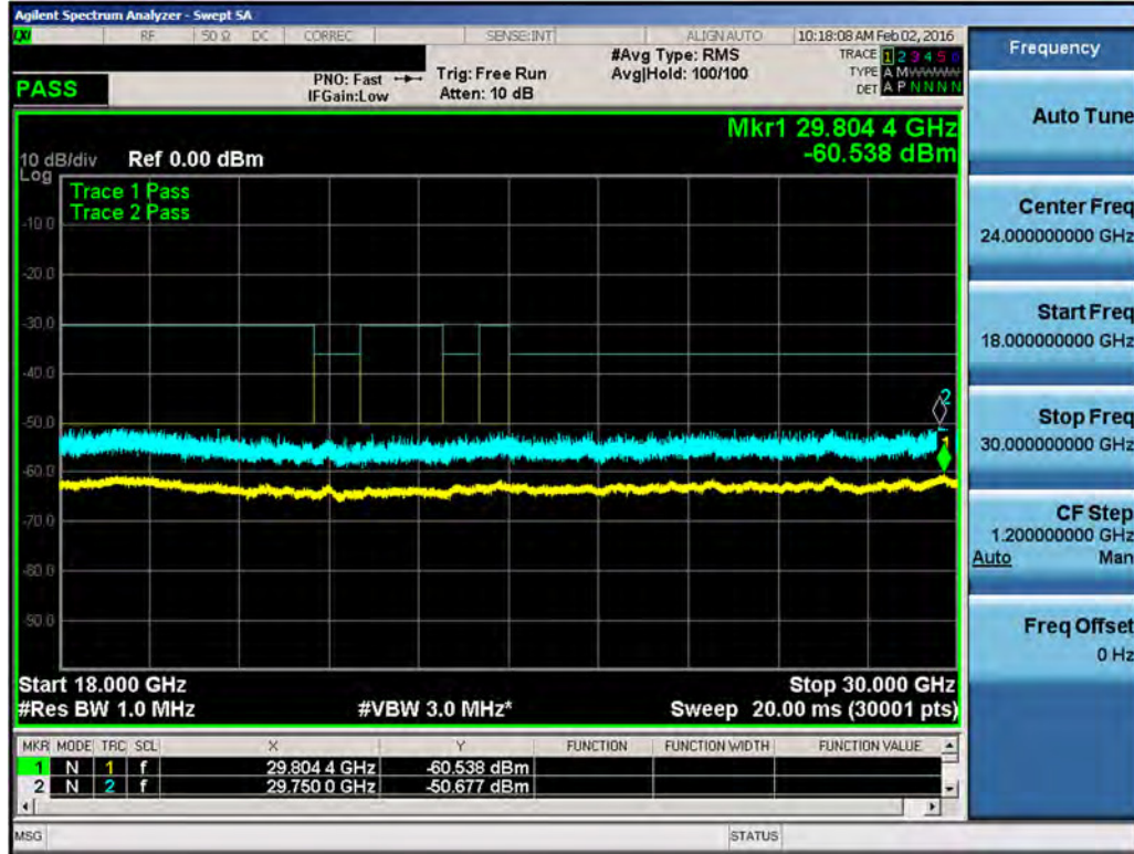
Plot 7-111. Conducted Spurious Plot (LAA (UNII Band 3, 40MHz BW) – Ch. 53340, 53540)
