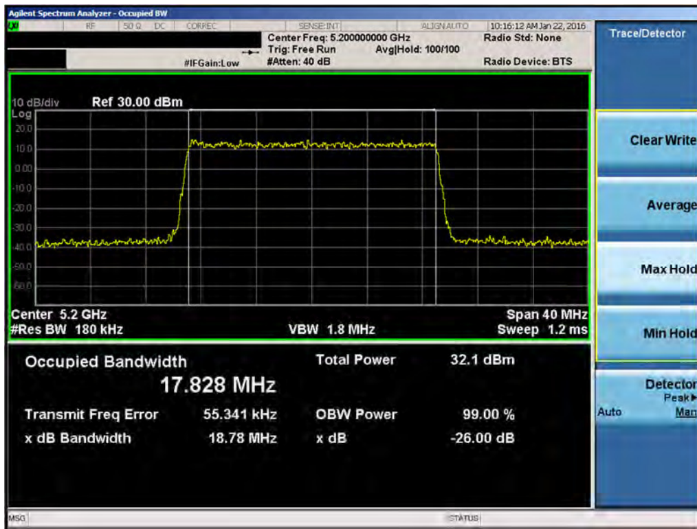
Plot 7-2. 26dB Bandwidth Plot (LAA (UNII Band 1, 20MHz BW) – Ch. 47290)
