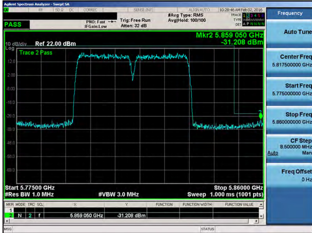
Plot 7-40. Conducted Peak Band Edge Plot #1 (LAA (UNII Band 3, 40MHz BW) – Ch. 53340, 53540)
