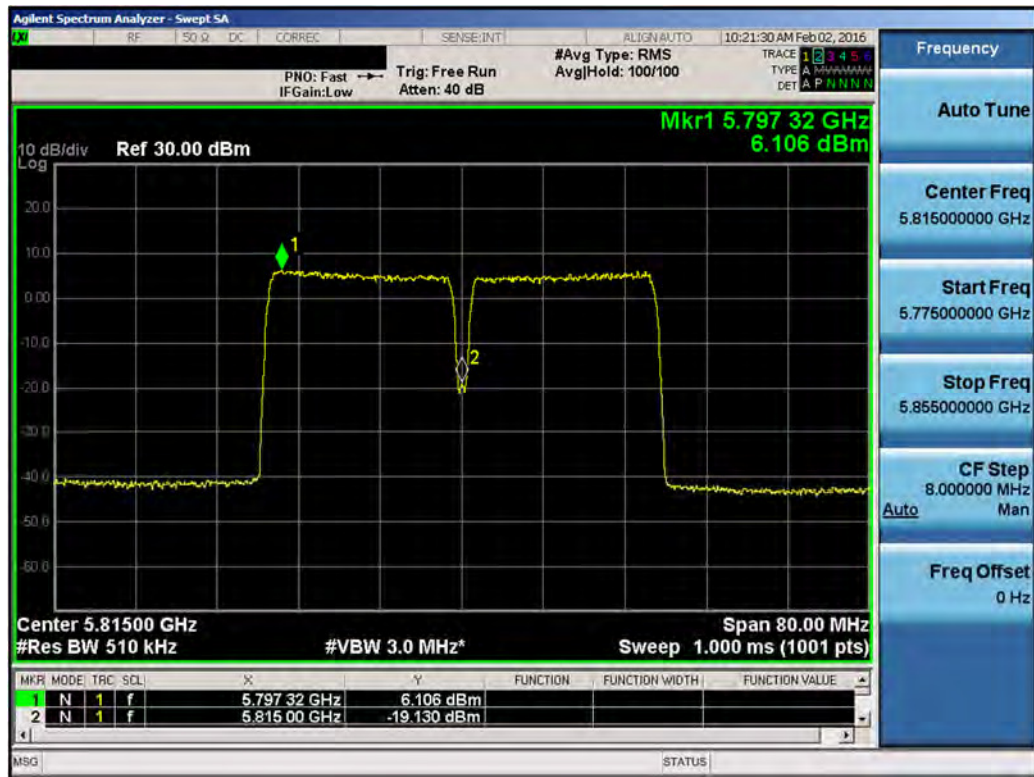
Plot 7-16. Power Spectral Density Plot (LAA (UNII Band 3, 40MHz BW) – Ch. 53340, 53540)
