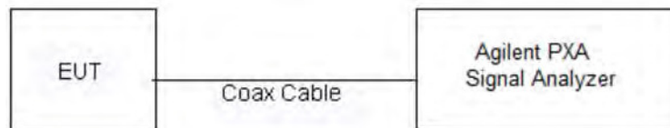
Figure 7-3. Test Instrument & Measurement Setup
