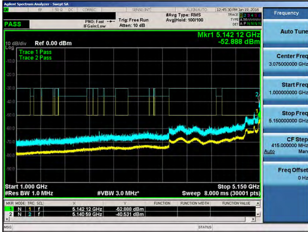
Plot 7-59. Conducted Spurious Plot (LAA (UNII Band 1, 20MHz BW) – Ch. 47290)
