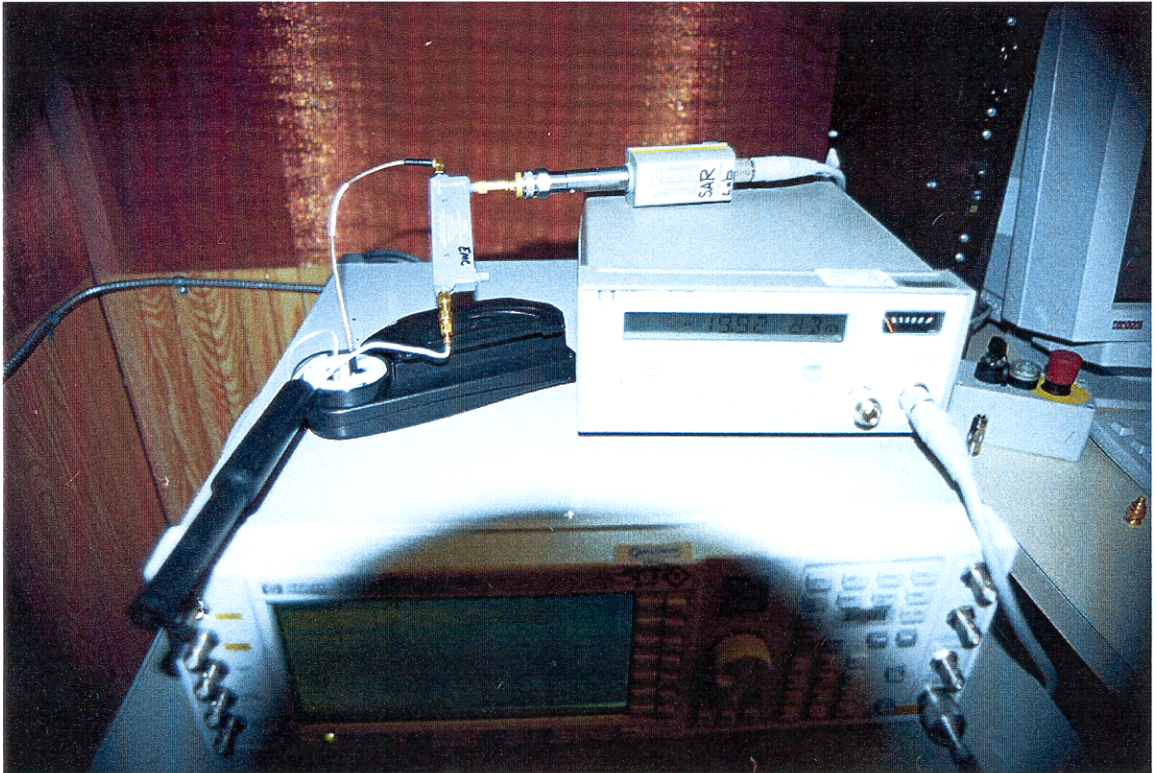
Photo 15 – GSP 610 Conducted Power Set-up
