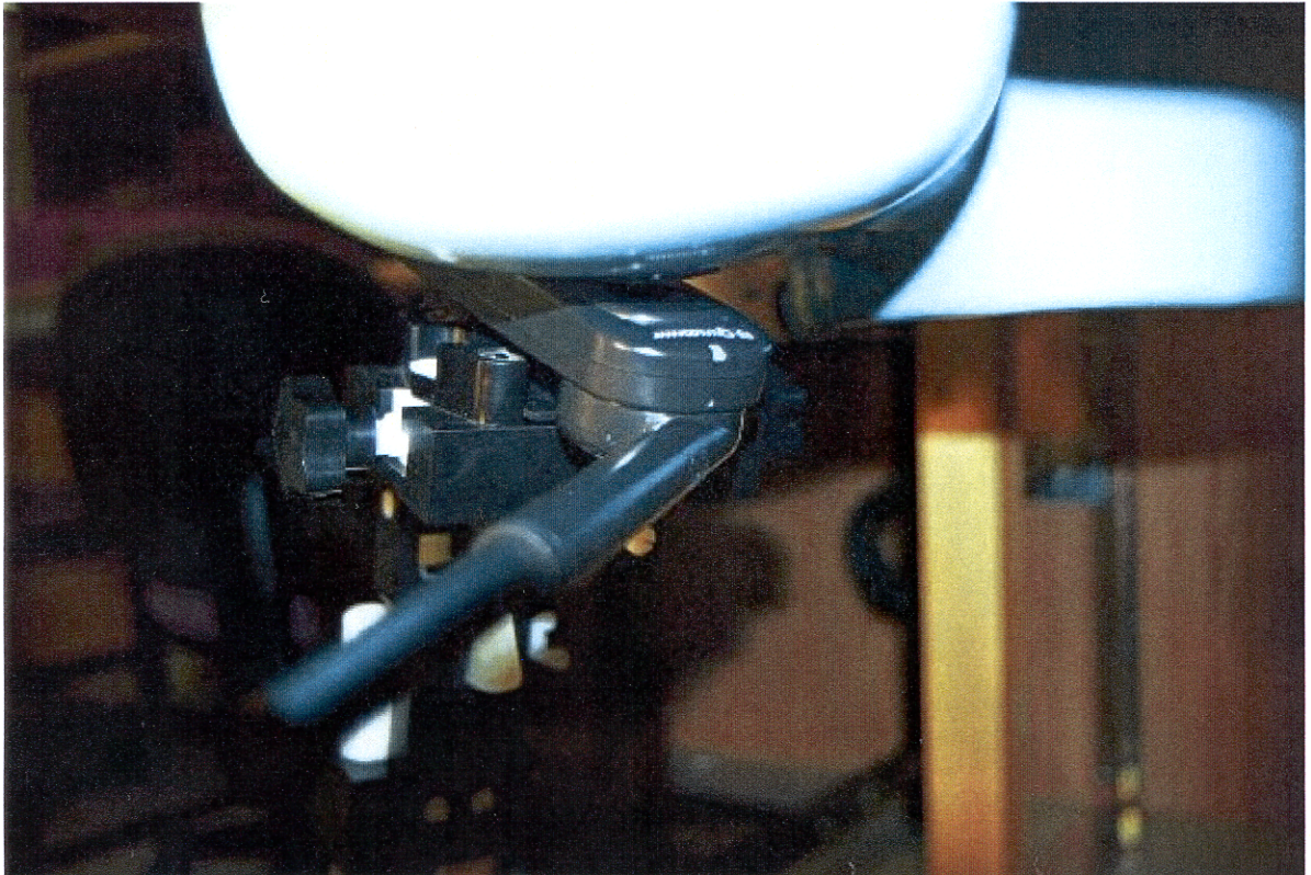
Photo 10 - SAR set-up: Bottom view, right side of head, correct antenna position
