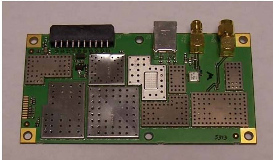
PCB With Shields In Place
