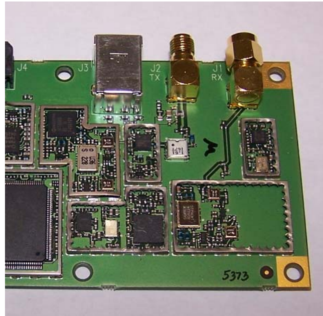
PCB Detail-Right Side
