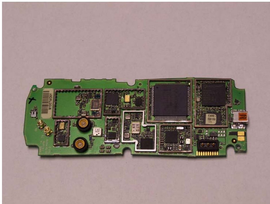
Figure 12 UT PCB Back Shields Open
