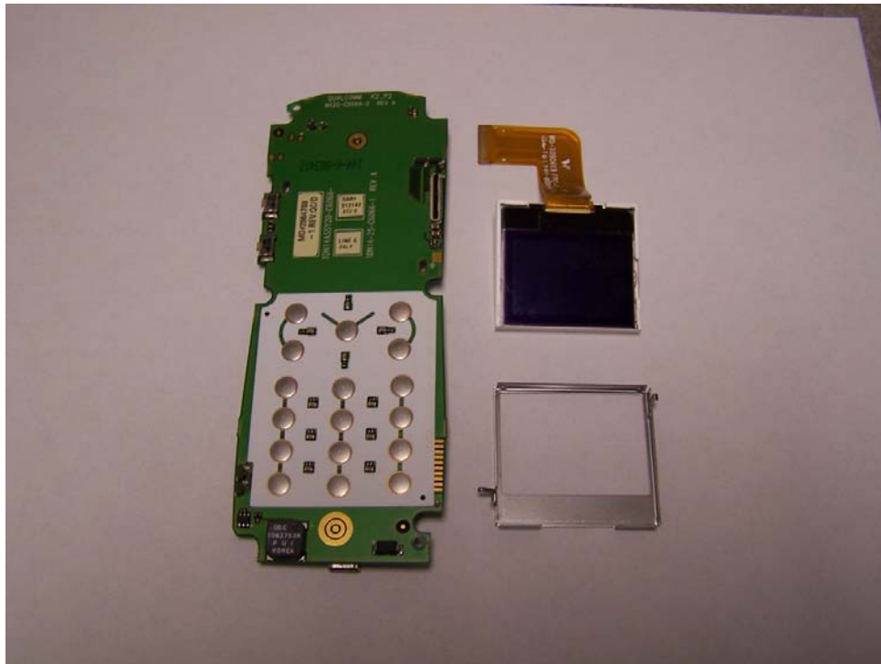
Figure 11 UT PCB Front LCD Removed
