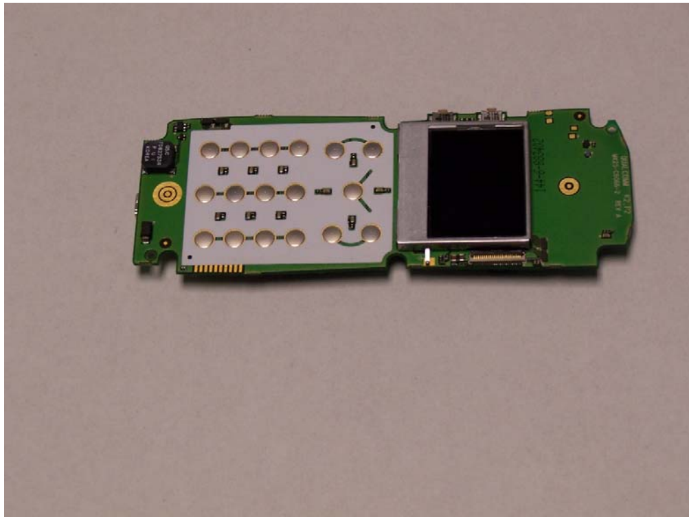
Figure 10 UT PCB Front with LCD
