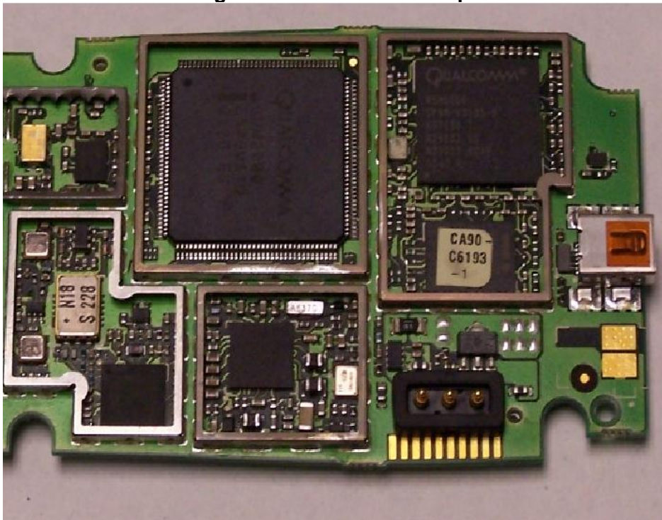
Figure 14 UT PCB Back Bottom Detail
