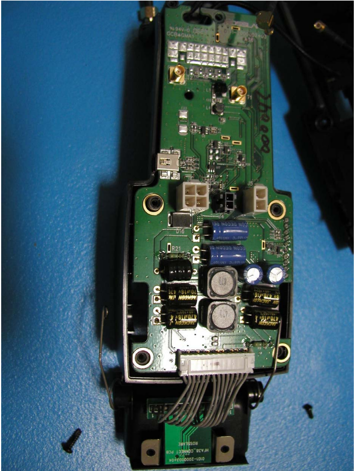
Figure 2 HFK Cradle Front
