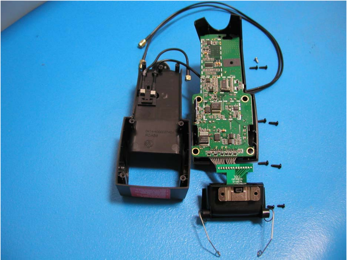
Figure 1 HFK Cradle Back
