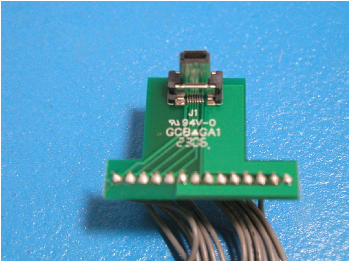
Figure 3 HFK Phone Connector Card
