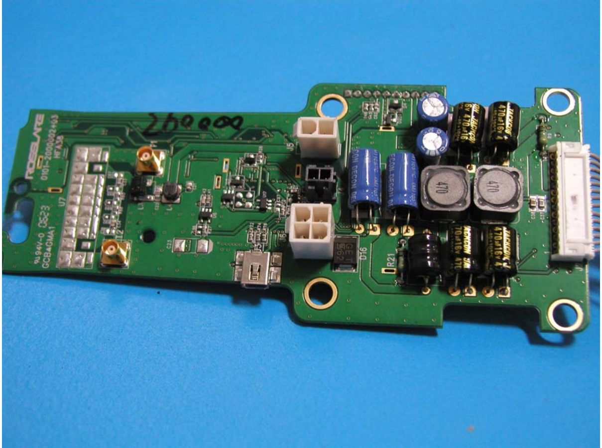
Figure 5 HFK PCB Front- Detail
