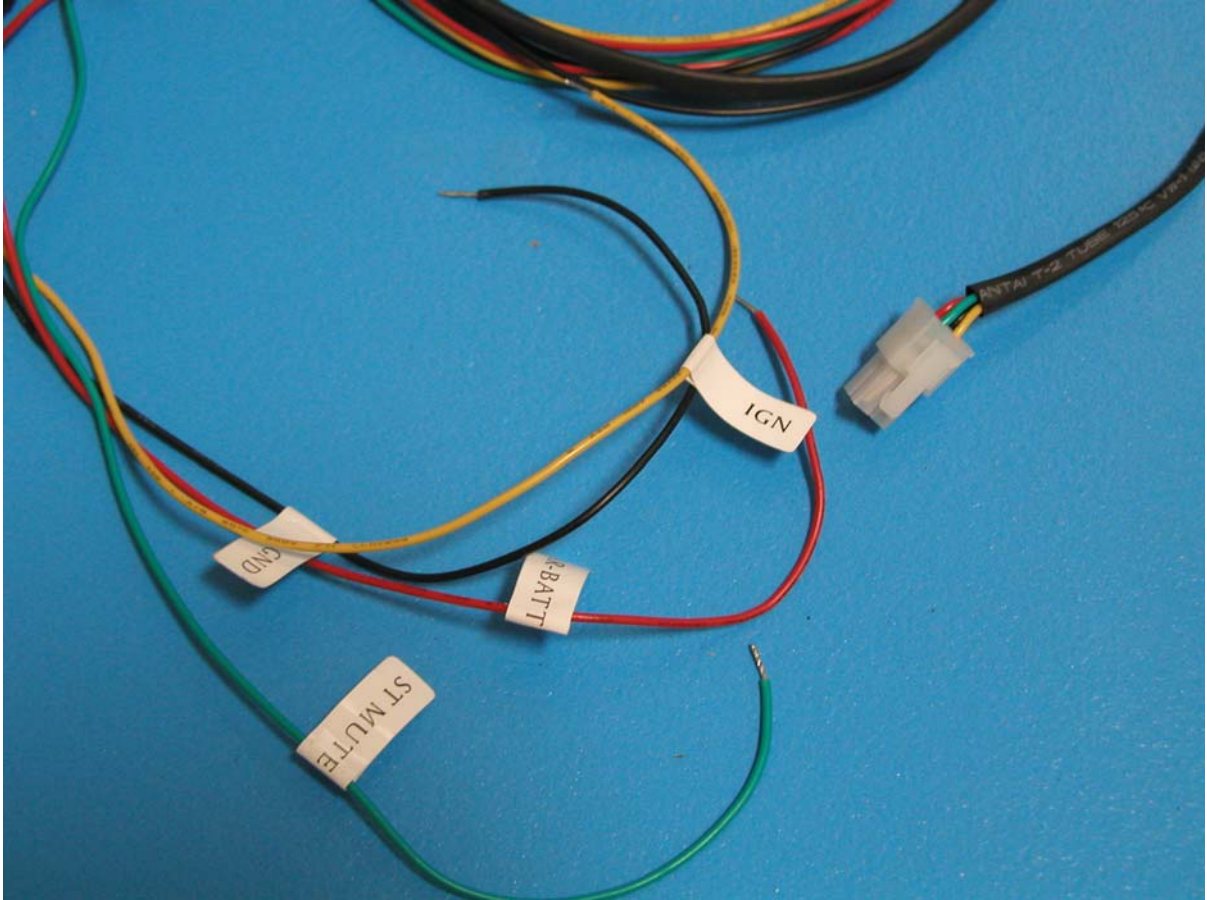
Figure 11 HFK External- Power Cable Detail
