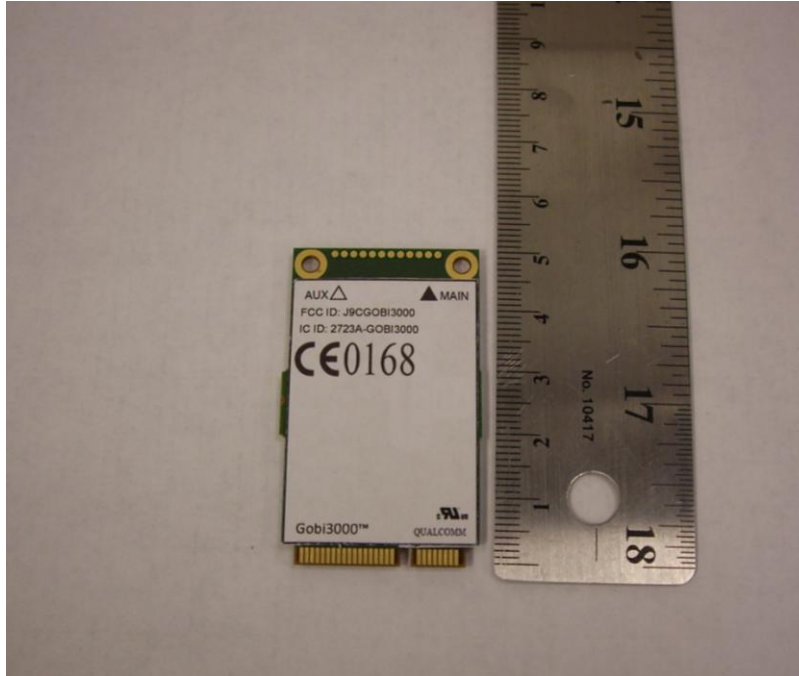
Figure 2 Gobi3000 Module Top View External Photograph
