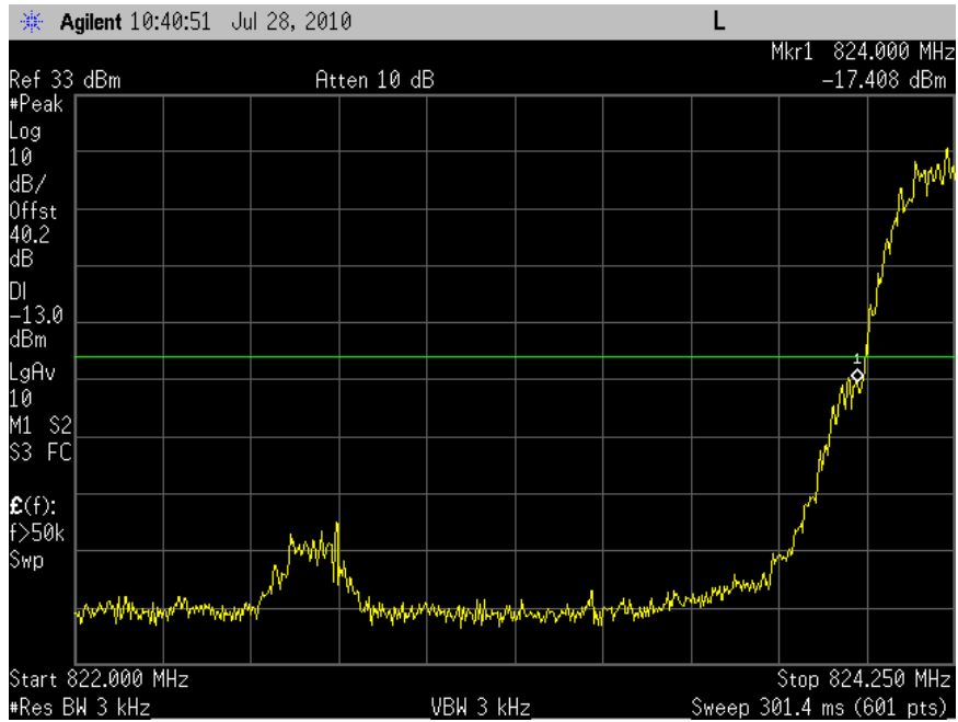
Plot 6.2 - 2 (Ch251, GMSK)
