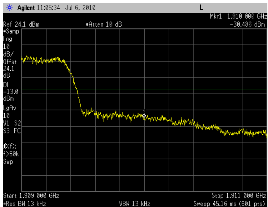
Plot 6.2-24 (Ch. 1175, RC3 SO55)
