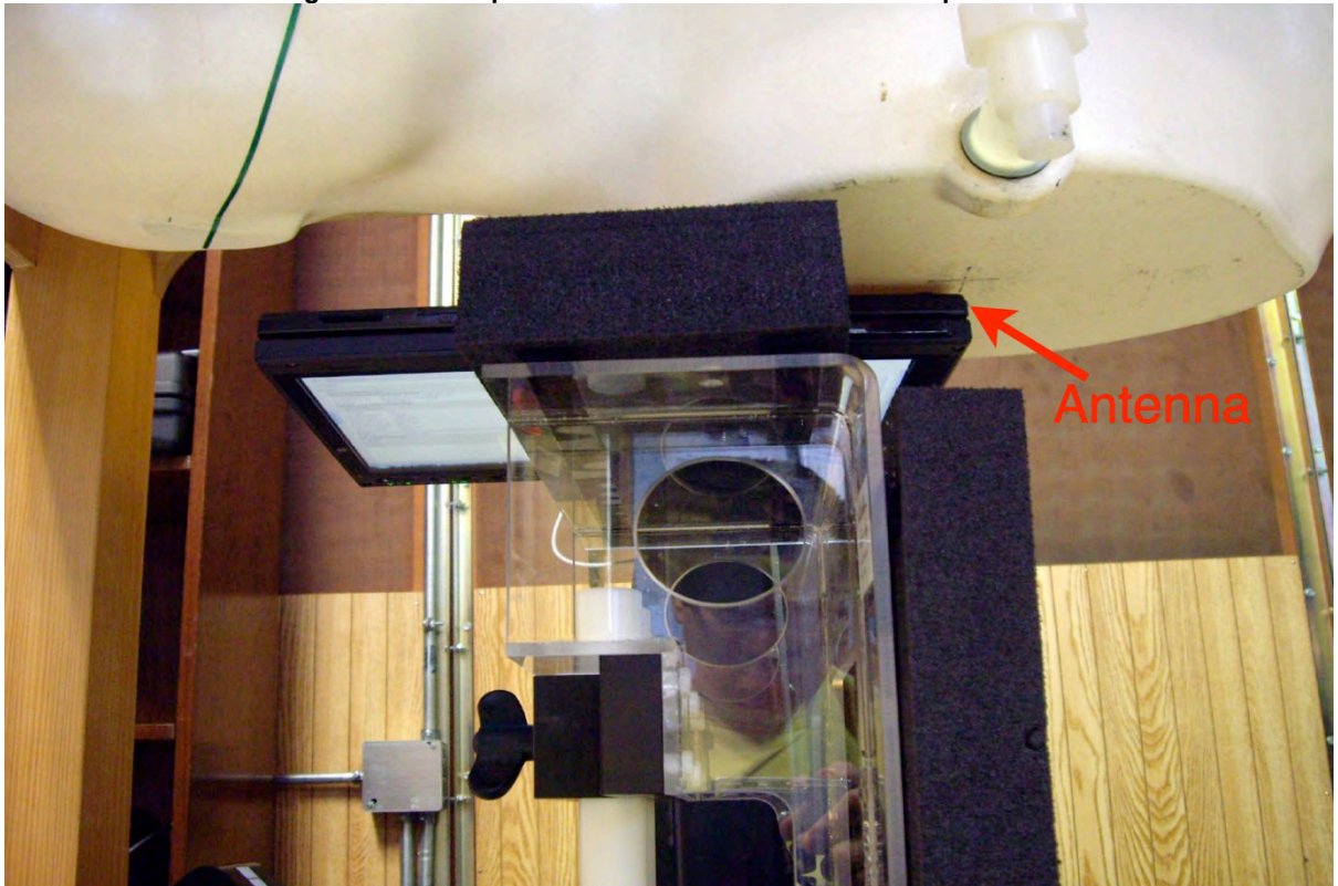
Figure 11-4 DUT positioned under Phantom – Tablet position
