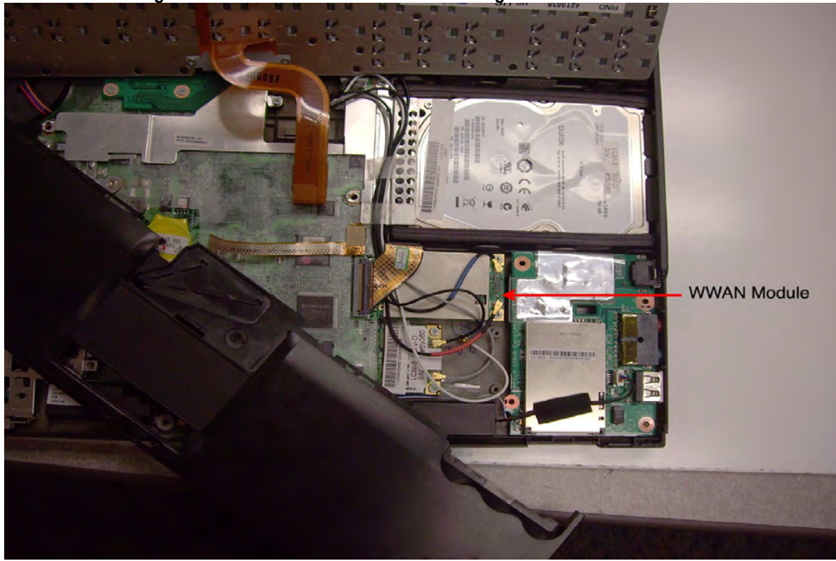
Figure 11-3 Bottom view of notebook showing WWAN module location
