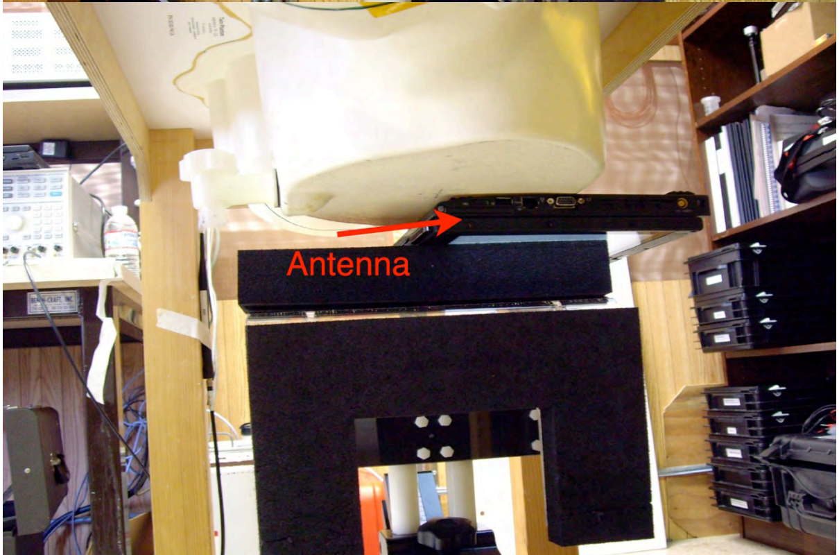
Figure 11-5 DUT positioned under Phantom – Secondary Portrait position
