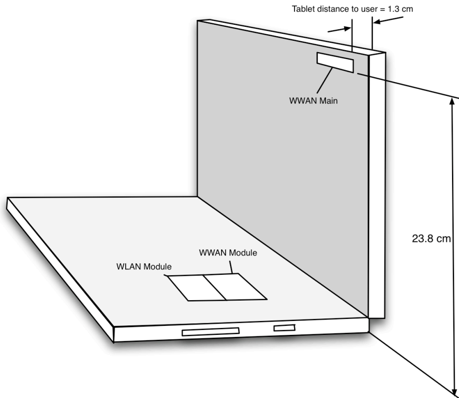
Figure 1-1 Antenna Locations
