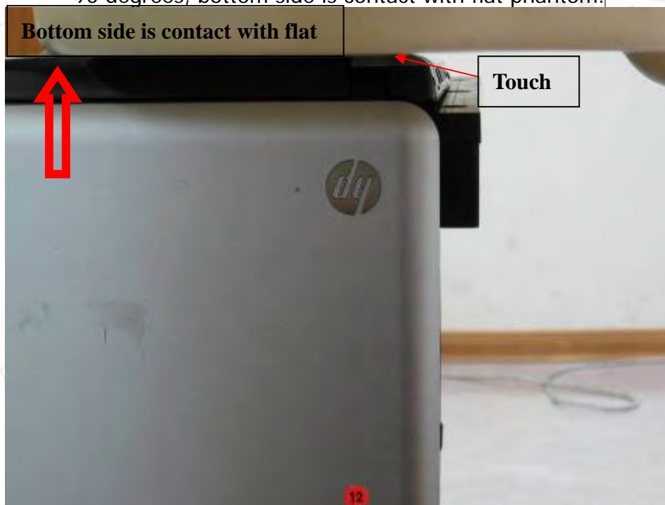
Fig.5 Bottom side of the Notebook is paralleled with flat phantom, open the panel with 90 degrees, bottom side is contact with flat phantom.
