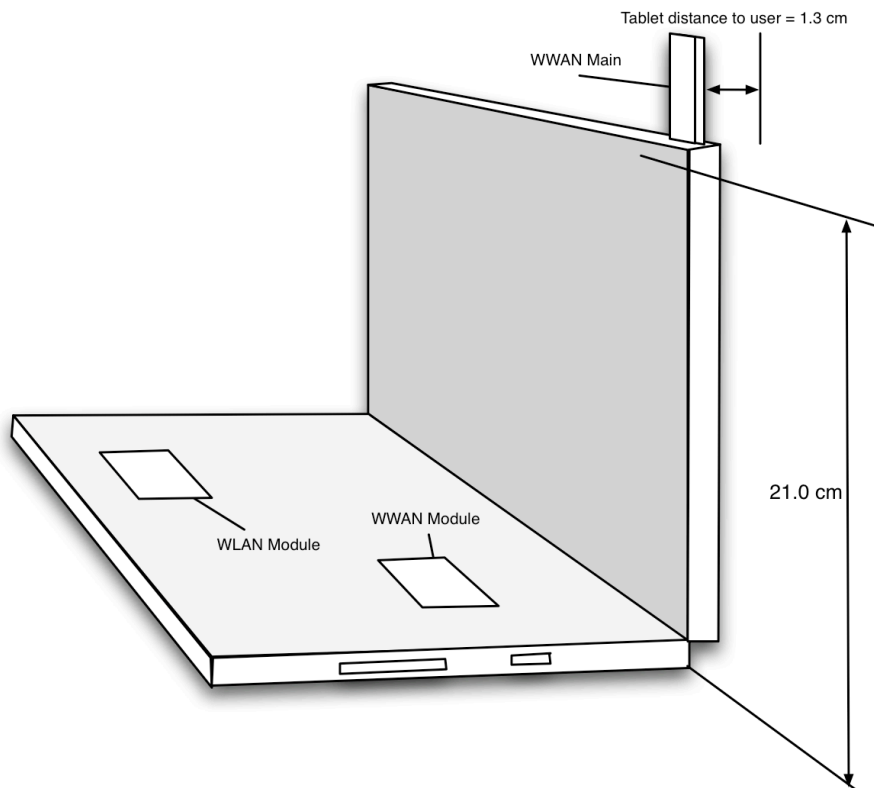
Figure 1-1 Antenna Locations
