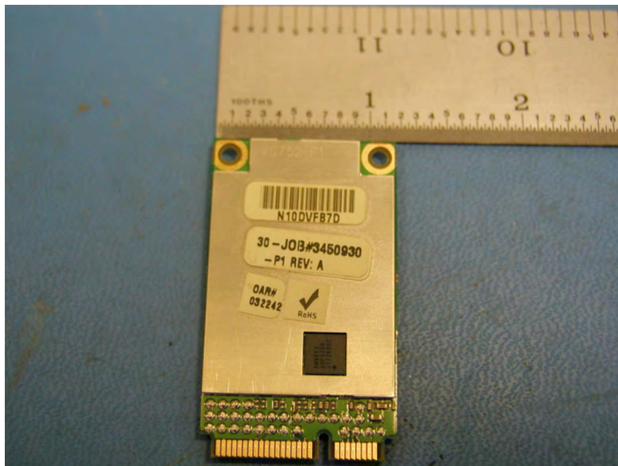
Figure 3 Gobi2000™ Module Rear External Photograph
