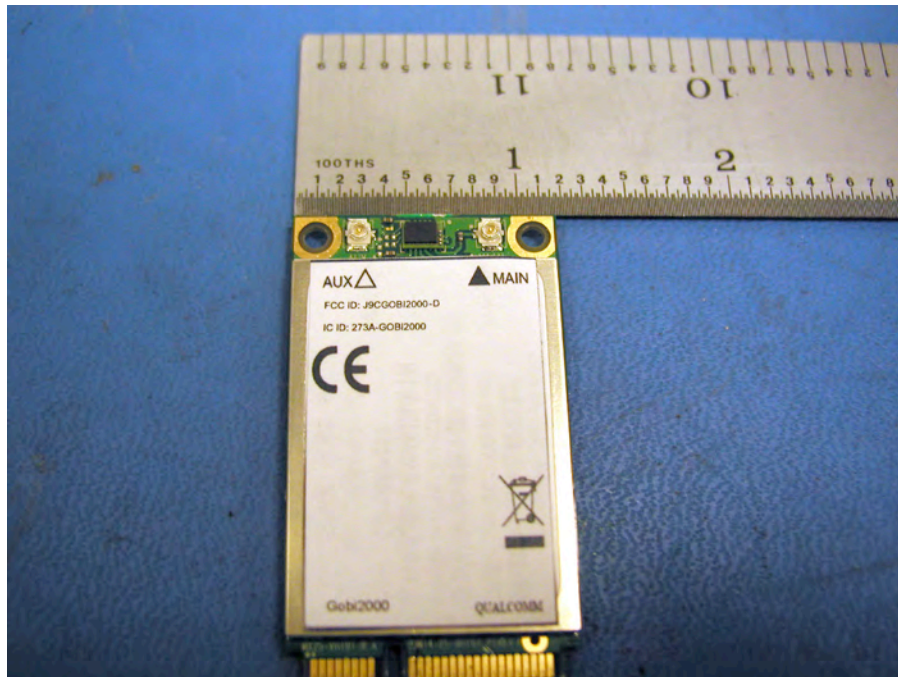
Figure 1 Gobi2000™ Module Label Location
