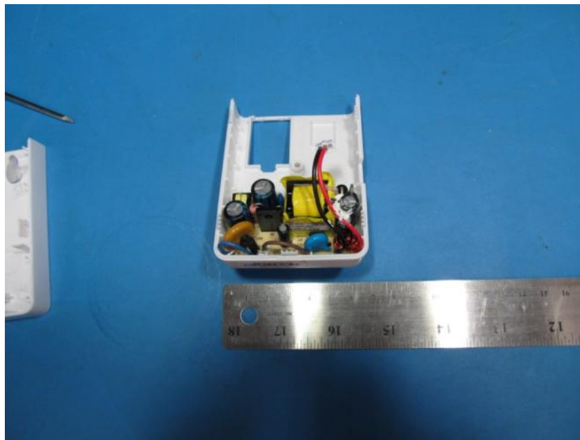
Figure 1-3: Rear Housing with power supply
