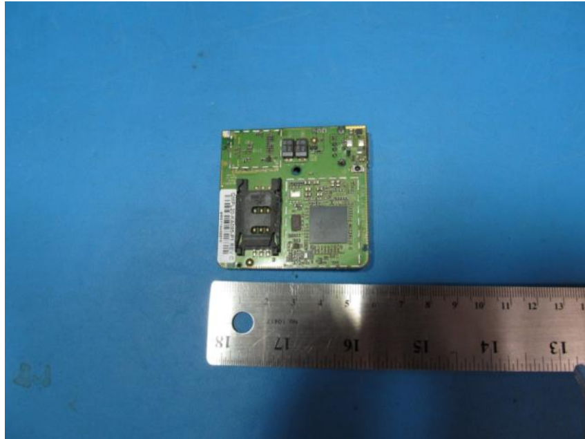
Figure 1-7: 2net board bottom with shields off
