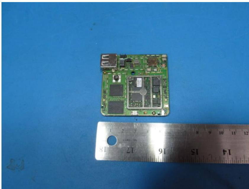
Figure 1-6: 2net board top with shields off
