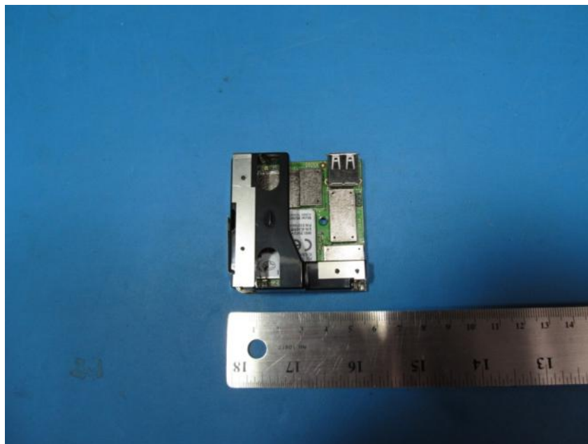
Figure 1-4: 2net board top with shields on
