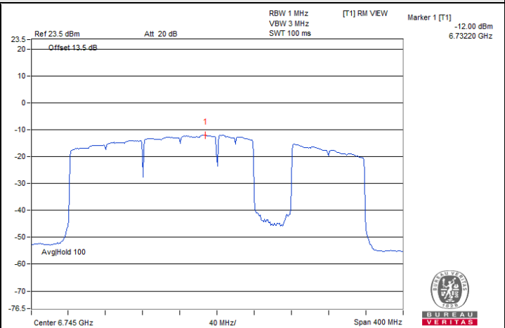
802.11be (EHT320) Punctured by 40 MHz / Chain 1 : CH 159@5
