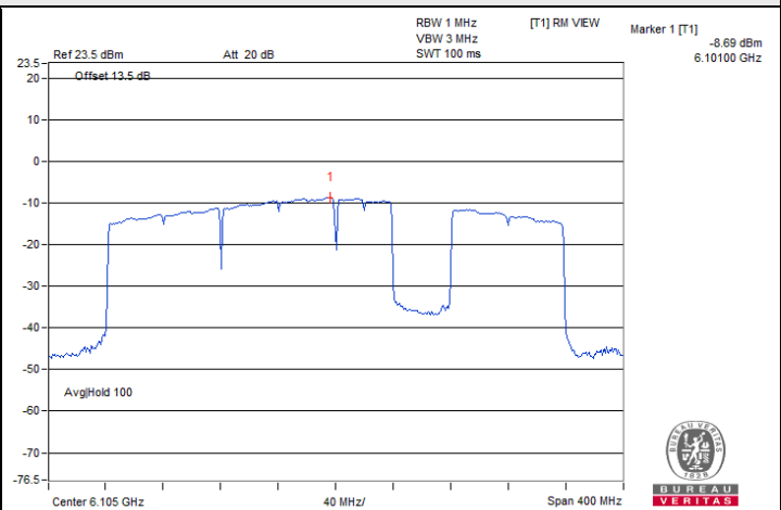
802.11be (EHT320) Punctured by 40 MHz / Chain 1 : CH 31@5
