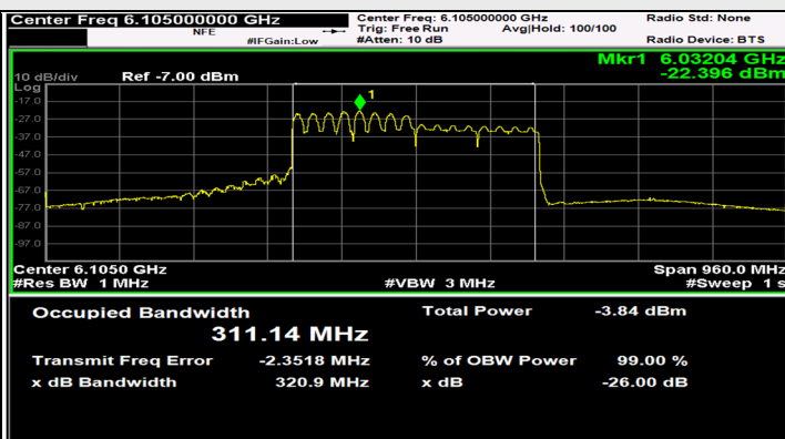
802.11be (HE320) / CH31
