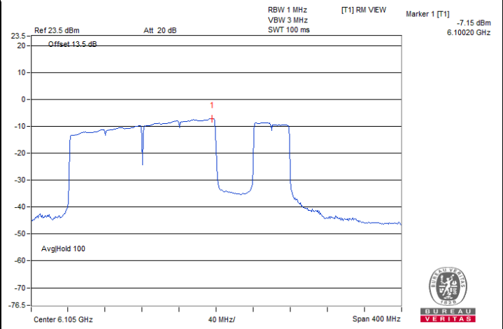
802.11be (EHT320) Punctured by 80+40 MHz / Chain 1 : CH 31@23
