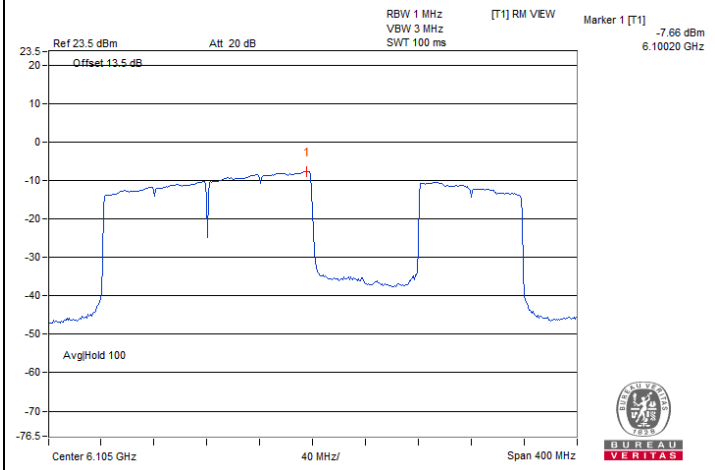
802.11be (EHT320) Punctured by 80 MHz / Chain 1 : CH 31@11
