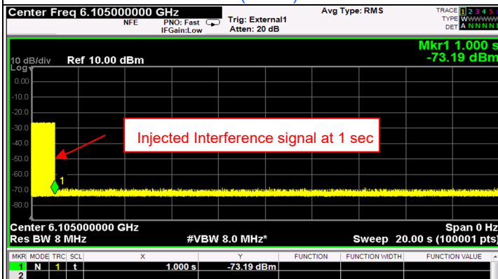
802.11be (HE320) / CH31(Middle)
