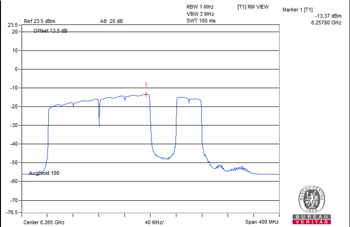
802.11be (EHT320) Punctured by 80+40 MHz / Chain 1 : CH 63@10
