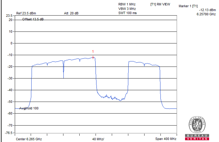
802.11be (EHT320) Punctured by 80 MHz / Chain 1 : CH 63@10
