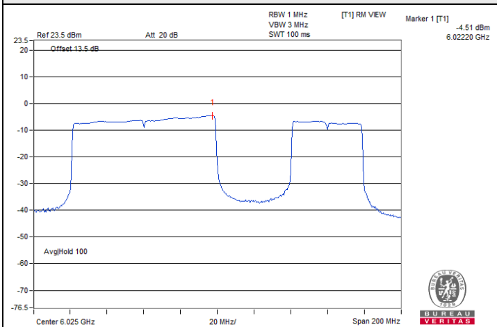
802.11be (EHT160) Punctured by 40 MHz / Chain 1 : CH 15@11
