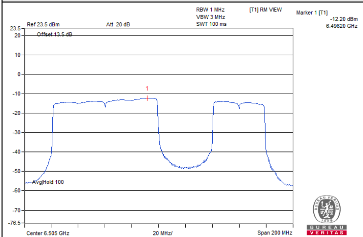
802.11be (EHT160) Punctured by 40 MHz / Chain 1 : CH 111@11
