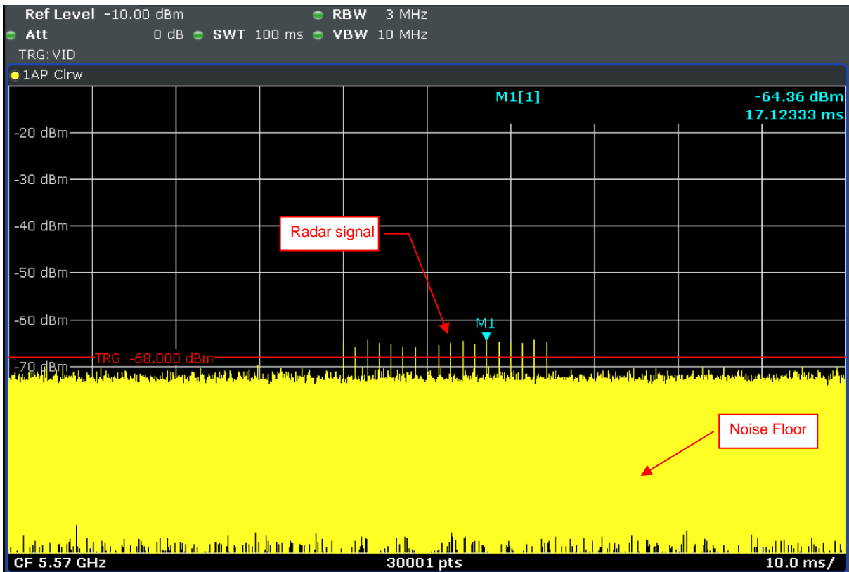
Radar Signal 0
