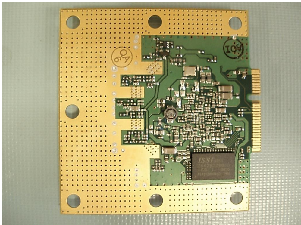
Figure 2 Bottom of the EA544D_1 Ethernet Adapter Card
