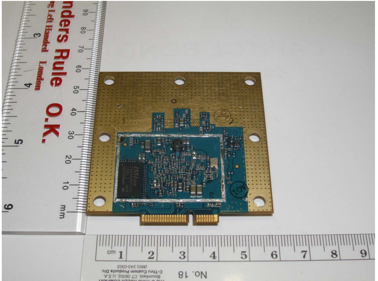
Figure 2 Bottom view of DC544D Family PCIe Daughter Card without shield
