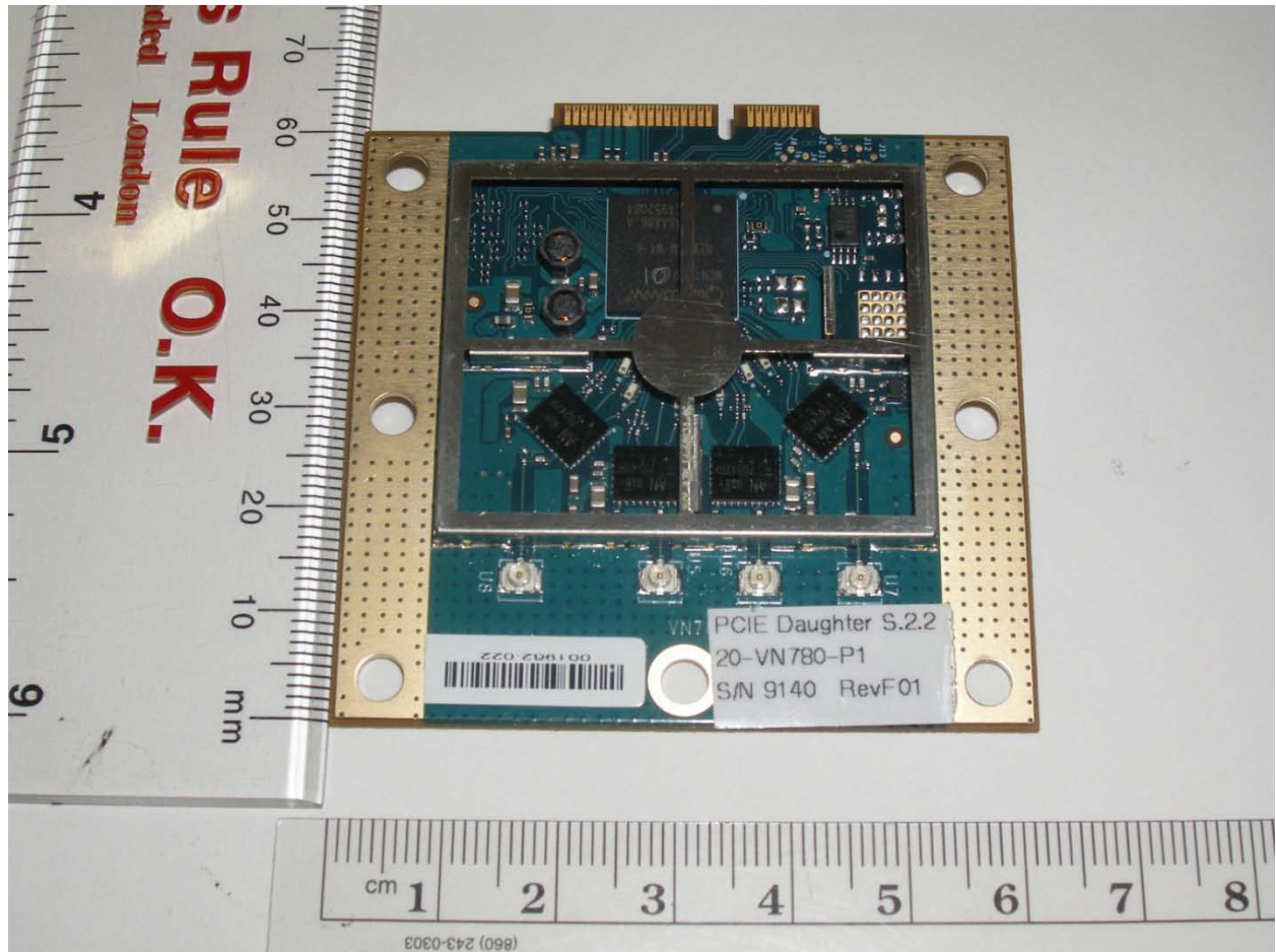
Figure 1 Top view DC544D Family PCIe Daughter Card without shield
