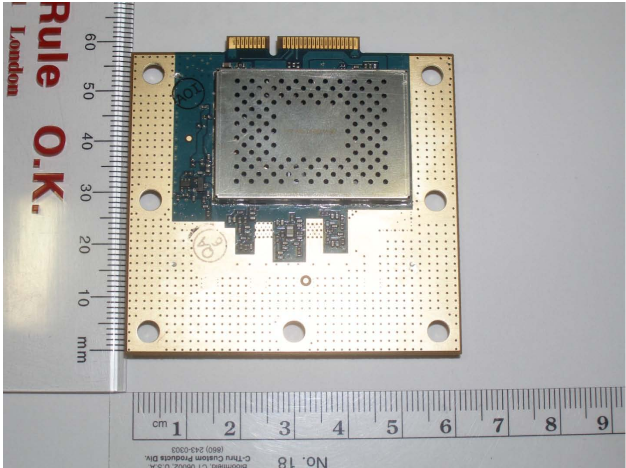
Figure 2 Bottom of DC544D Family PCIe Daughter Card with shield
