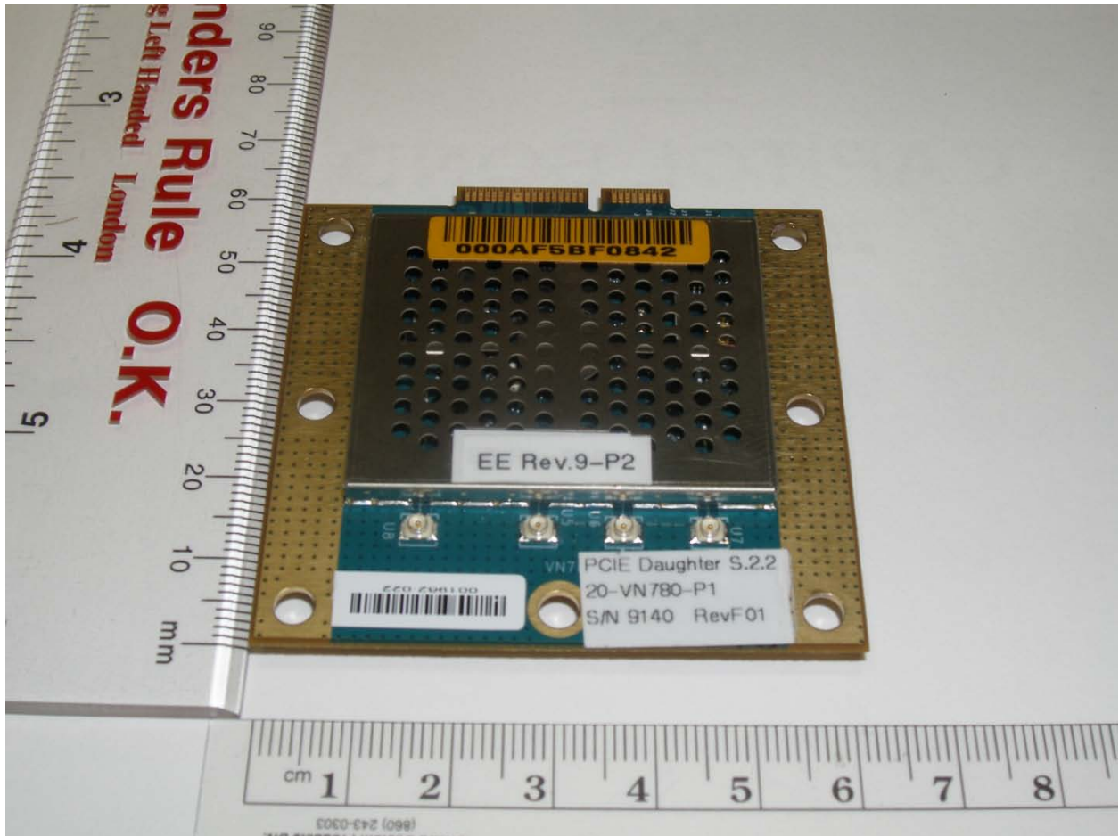
Figure 1 Top view DC544D Family PCIe Daughter Card with shield
