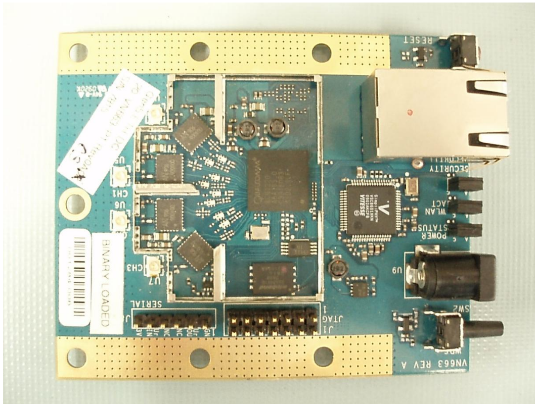
Figure 1 DC544D_1 PCIe Daughter Card without shield
