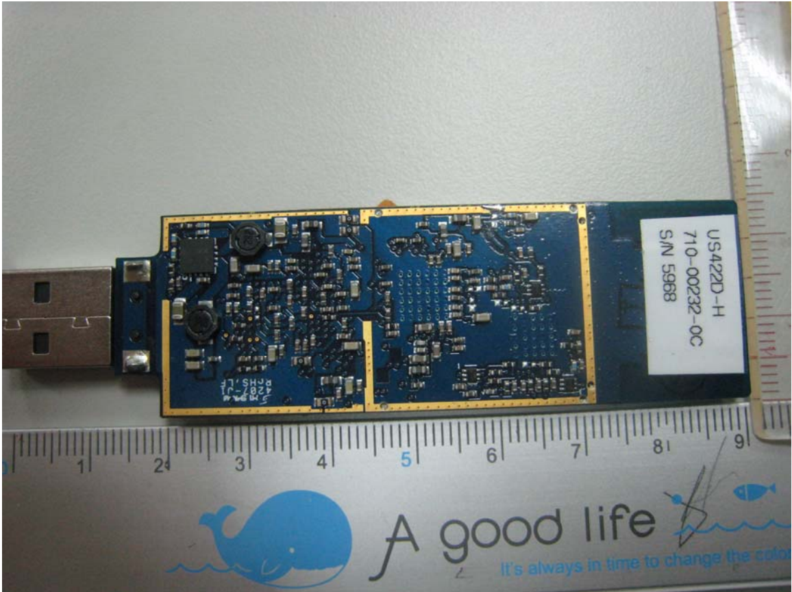
Internal view, Bottom side 65-VF438-P2 (US422D_H) FCC ID: J9C-65VF438P2
