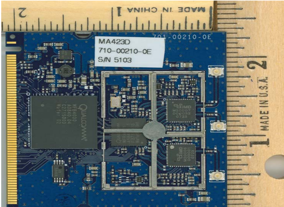
Internal view, Top side 65-VF320-P2 (MA423D_H) FCC ID: J9C-65VF320P2
