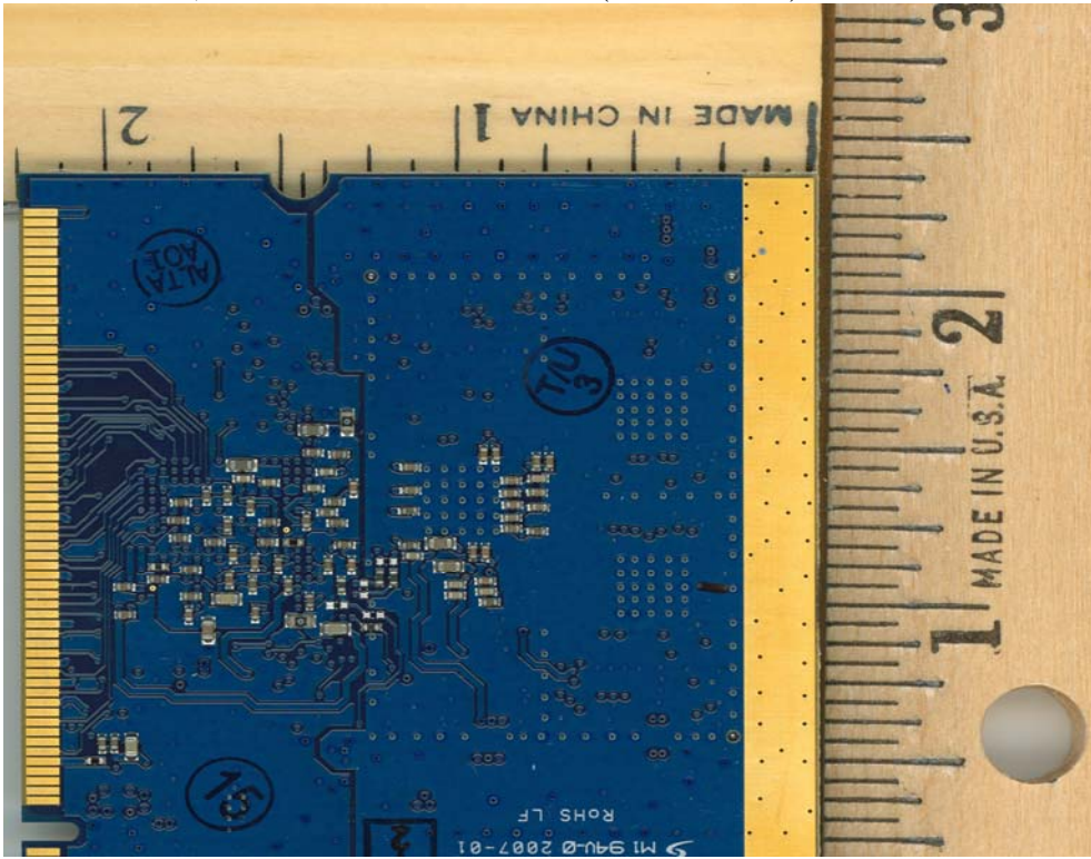
Internal view, Bottom side 65-VF320-P2 (MA423D_H) FCC ID: J9C-65VF320P2
