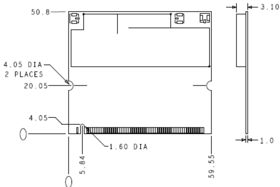
Figure 3 PCB and Shield Mechanical Drawing (dimensions in millimeters)
