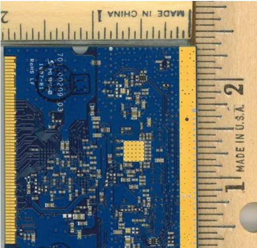
Internal view, Bottom side 65-VE240-P1 (MA423GD) FCC ID: J9C-65VE240P1
