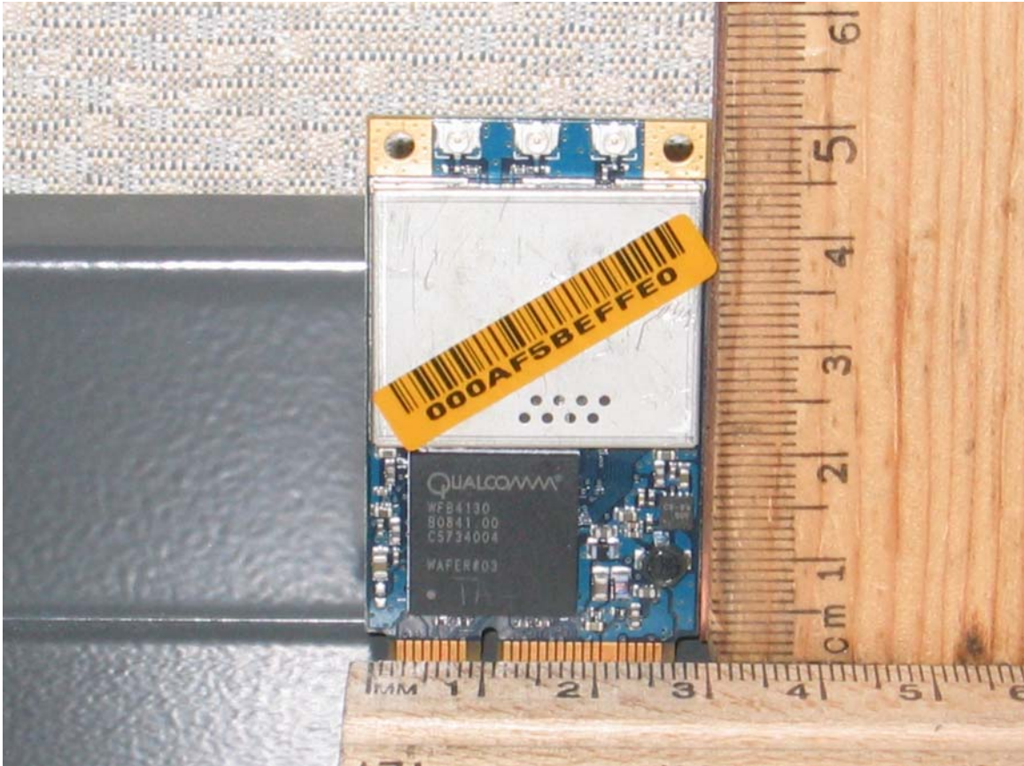
External view, Top side 65-VE239-P2 (MC423D_H) FCC ID: J9C-65VE239P2
