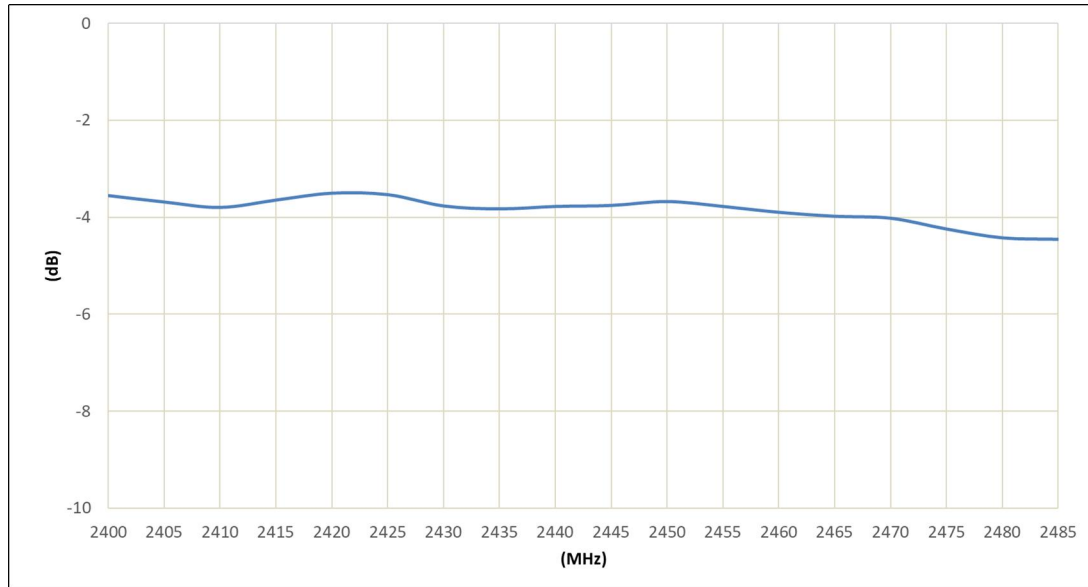
c) Average Gain (dB)
