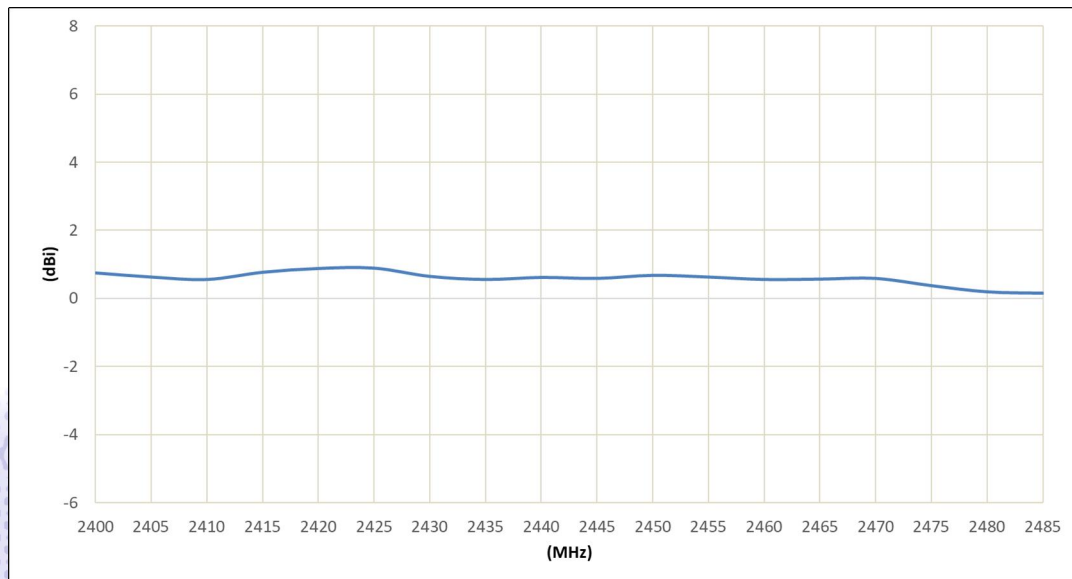
d) Peak Gain (dBi)
