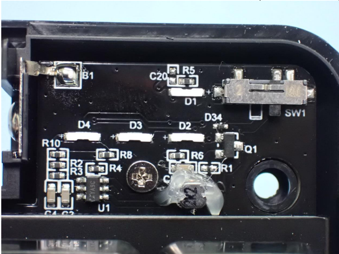
Figure 11 Internal View (PCB, Zoom View)
