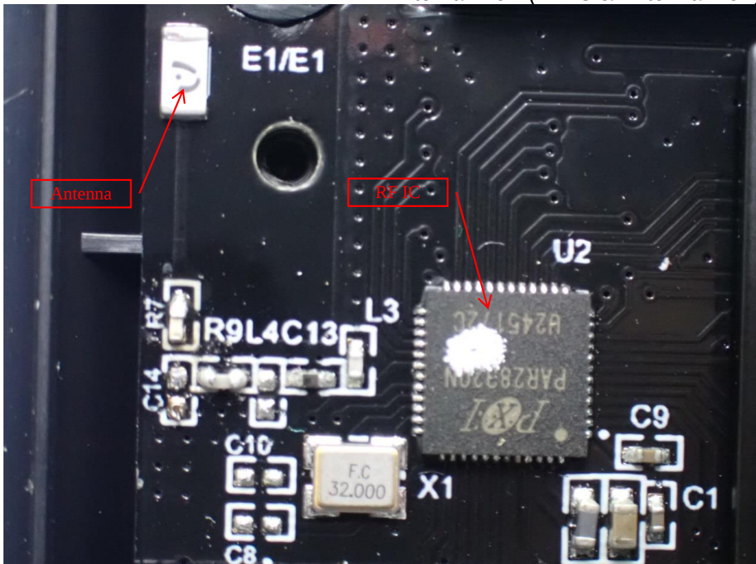
Figure 10 Internal View (RF IC & Antenna View)
