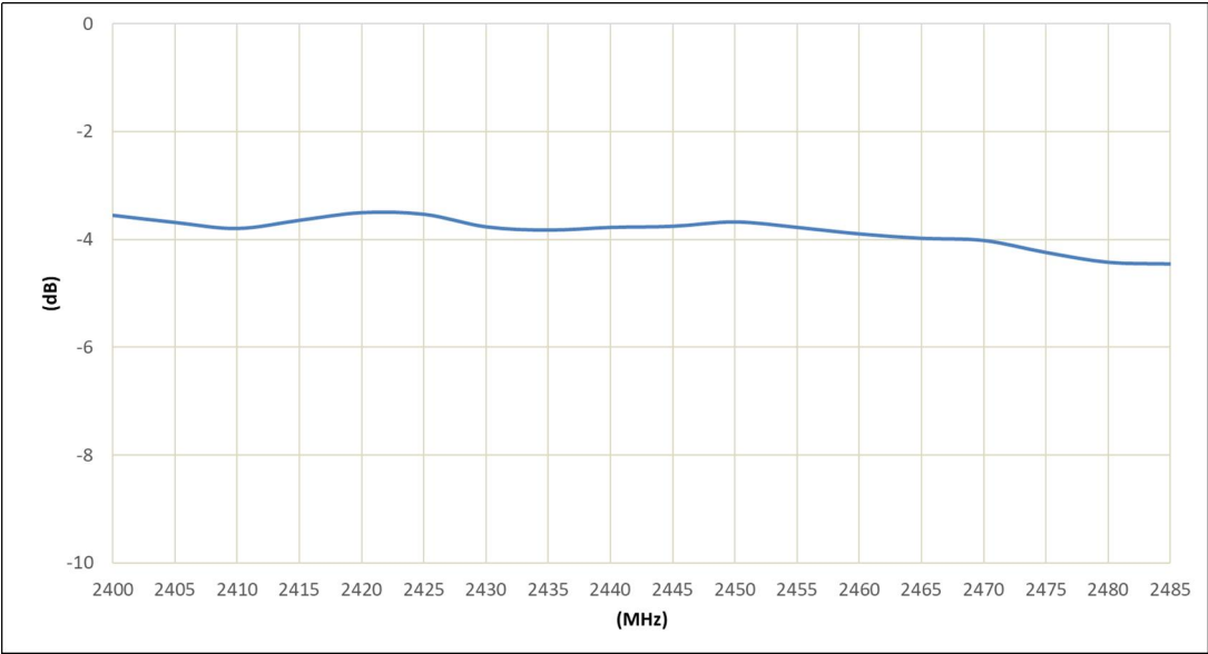
c) Average Gain: Max. -3.8dBi
