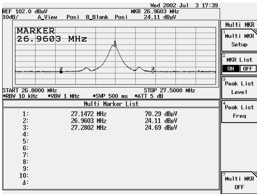
Figure Channel 1: (Horizontal)
