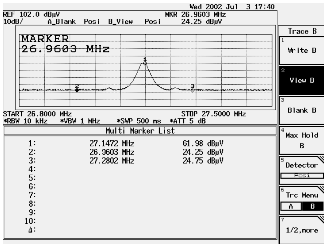
Figure Channel 2: (Vertical)
