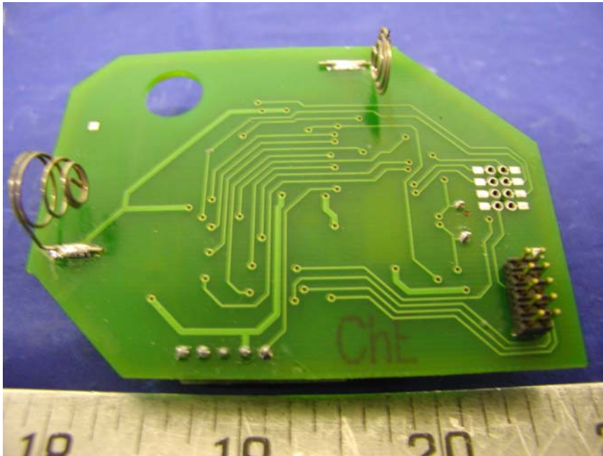
Transmitter Main Board - Solder View
