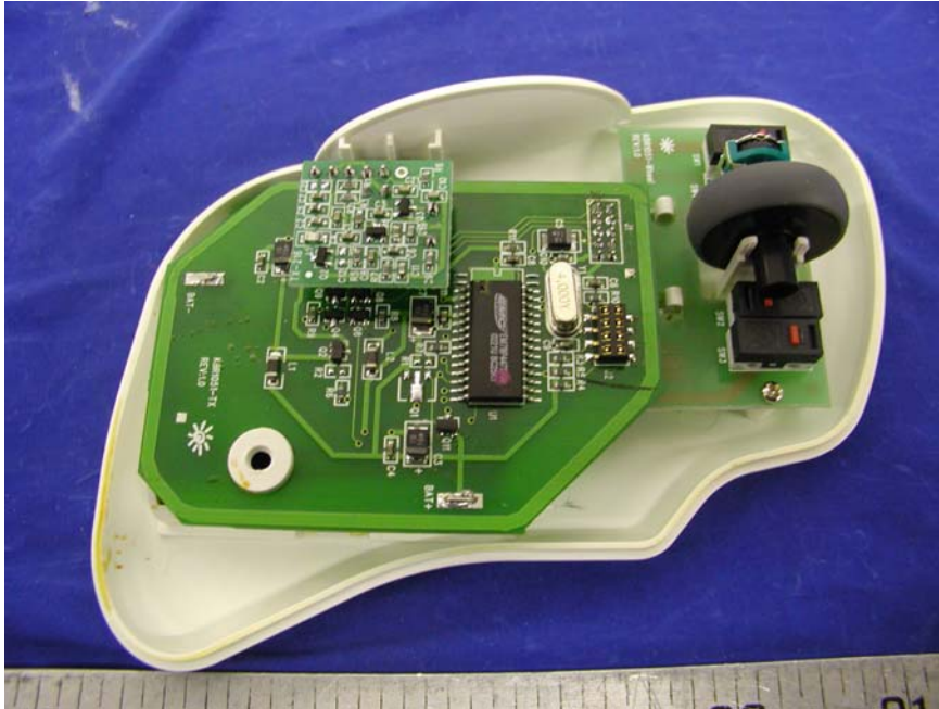
Transmitter Main Board - Component View 1
