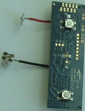
CB942A - battery wires and mechanical switches
