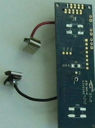
CB942 - battery wires and membrane switch
