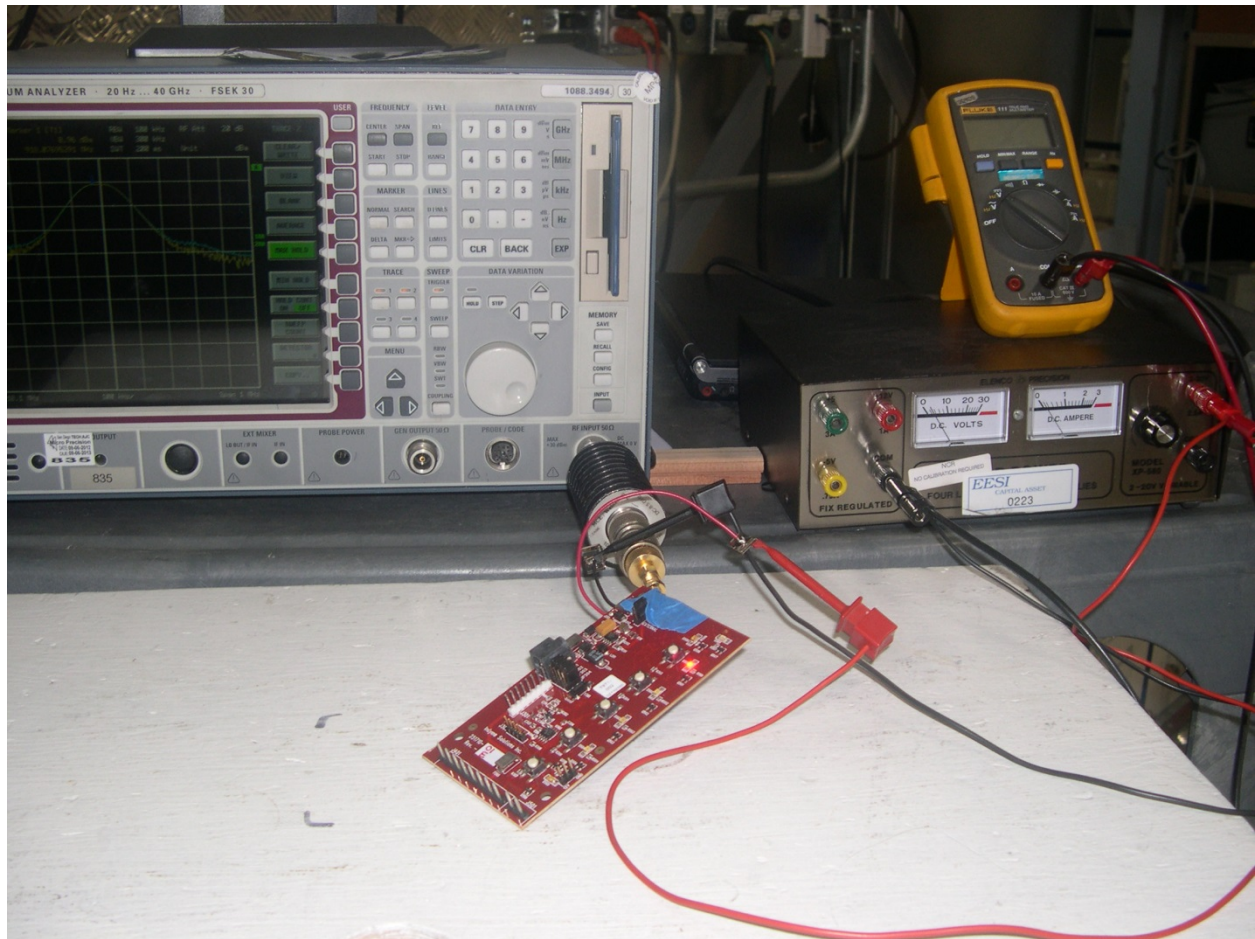
Pigtail added for conducted power, spurious
