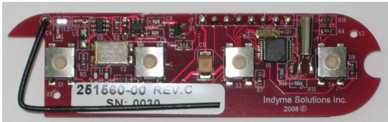
PCB Front
